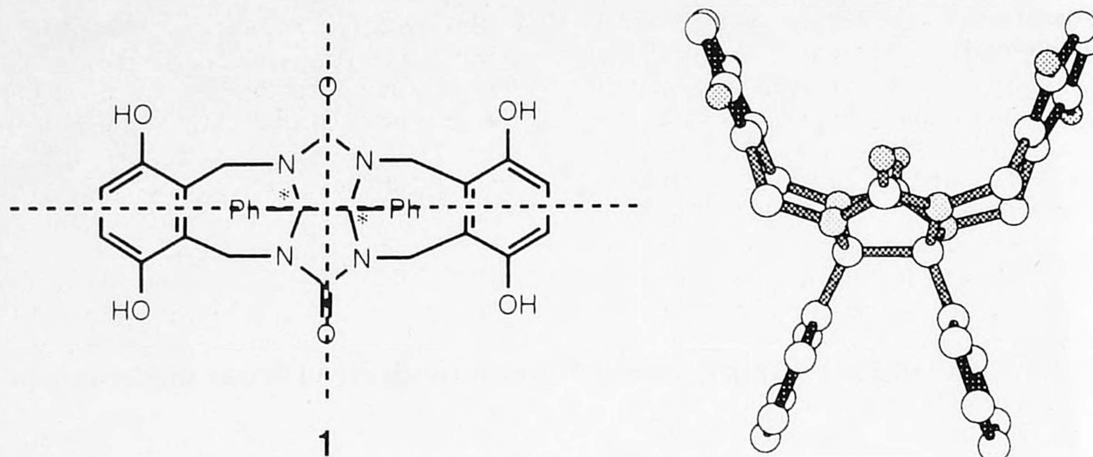
Figure 1. Division of compound 1 into four quadrants (left) and the X-ray structure of this compound (right).
