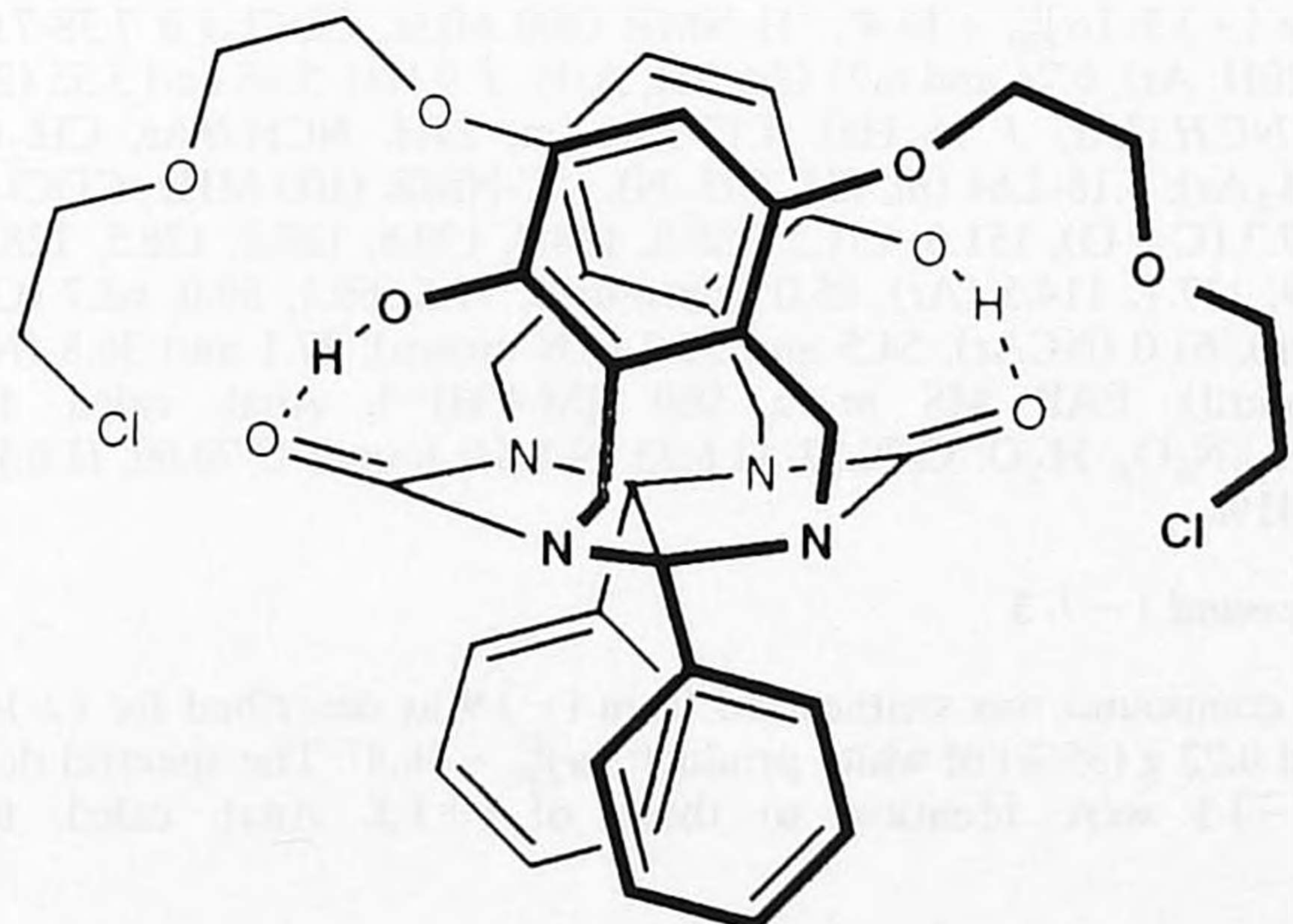
Figure 4. The optimization of the hydrogen bonds in 10 by a twist in the molecule.
