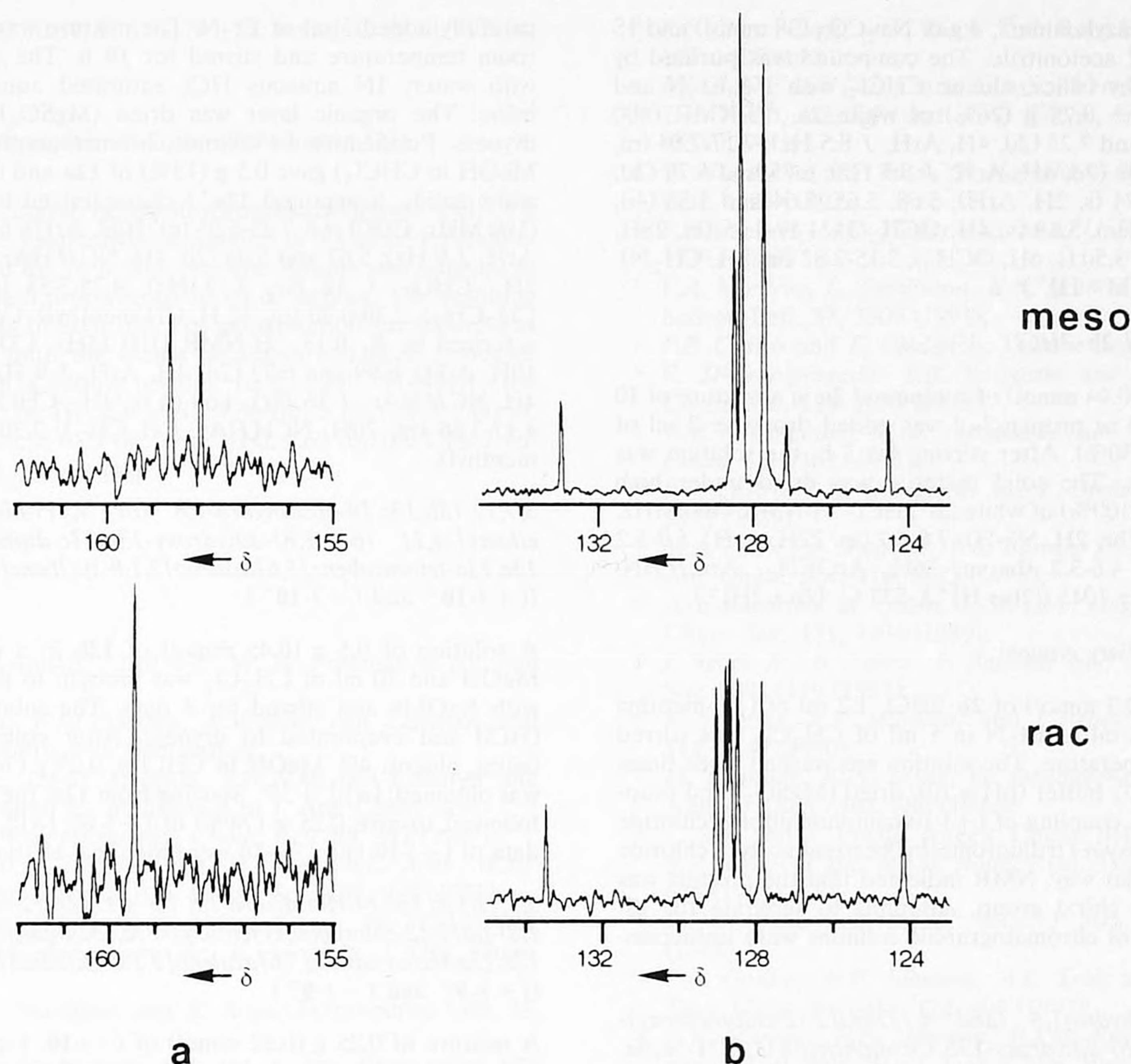
Figure 3. Low-field regions (a) and aromatic regions (b) of the ^{13}\text{C} -NMR spectra of meso-11 (above) and rac-10 (below).
