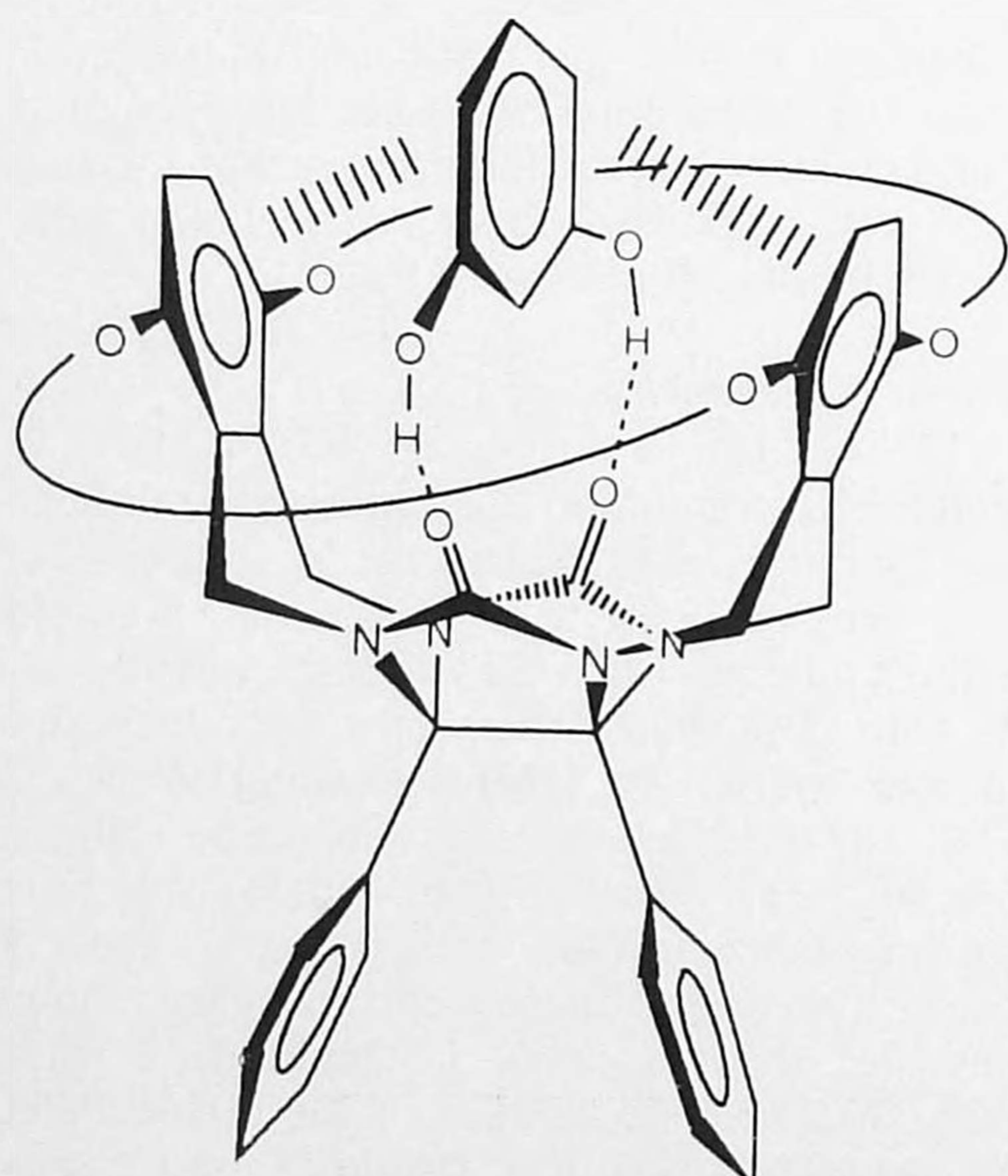
Figure 2. Schematic representation of the binding of benzene-1,3-diol in the basket-shaped receptor molecule based on 1.
