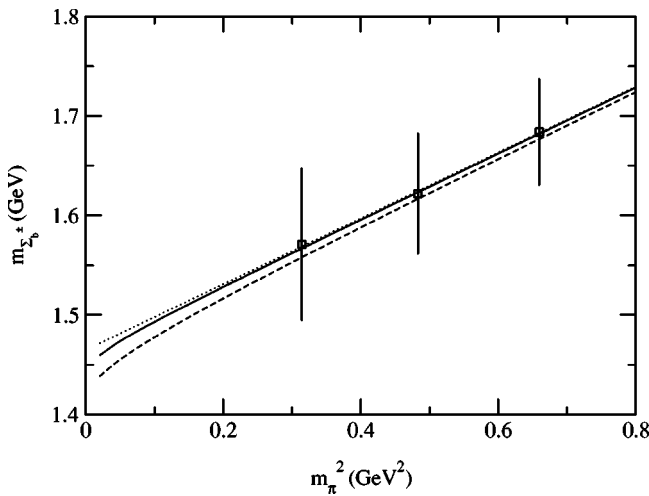
FIG. 5. Phenomenological fits to the lattice data for the masses of \Sigma_b^{*\pm} as a function of the pion mass. The solid (dashed) line corresponds to \Lambda=0.4 (0.6) GeV with finite lattice volume effects being taken into account and the dotted line represents the fit using a linear extrapolation.
