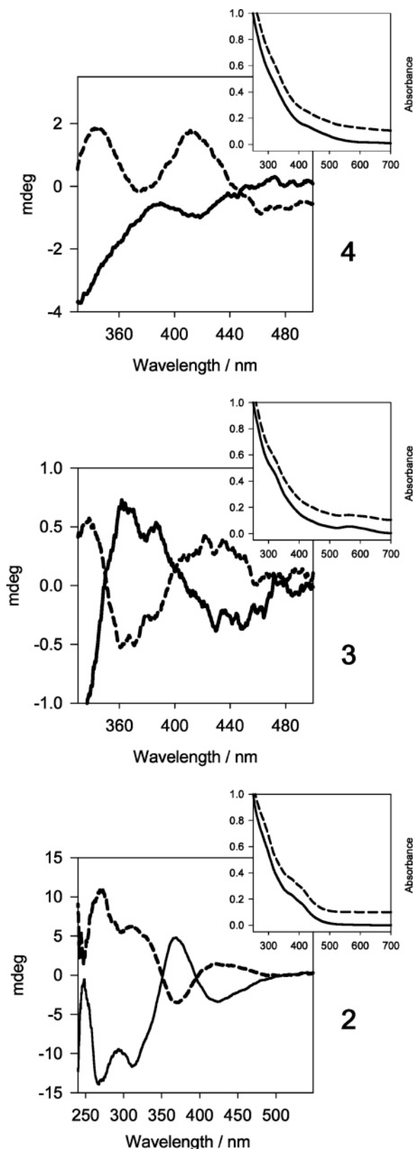
Figure 8. CD and UV-vis spectra of separated compounds 2–4 of gold particles covered with N -isobutyryl- L -cysteine (dashed) and N -isobutyryl- D -cysteine (solid line). The UV-vis spectra were scaled to 1 absorbance unit at 250 nm.
