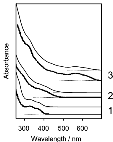
Figure 7. Comparison between UV-vis spectra of separated gold N -isobutyryl-L-cysteine compounds 1–3 (see Figure 5) and corresponding L-glutathione compounds reported in ref 50 (with permission from the American Chemical Society).
