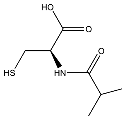
Chart 1. Structure of N -Isobutyryl-L-cysteine
