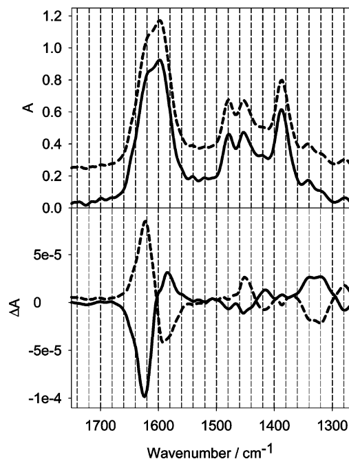
Figure 1. Infrared (top) and VCD (bottom) spectra of N -isobutyryl-cysteine protected gold nanoparticles in NaOH/D 2 O. Solutions were made from 7 mg of sample in 50 μL of solution. The dashed (solid) lines correspond to the spectra of the particles covered by the L-enantiomer (D-enantiomer). The IR spectrum of the particles covered with N -isobutyryl-L-cysteine was offset for clarity. See Experimental Section for more details.
