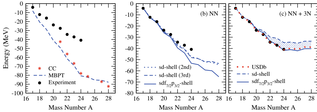
Fig. 1. Ground-state energies of neutron-rich oxygen isotopes relative to ^{16}\text{O} , with experimental energies from the AME 2003 atomic mass evaluation [36]. Panel (a) compares results calculated in MBPT to those from CC theory based on the same low-momentum NN interactions. The MBPT results are based on the SPEs obtained in CC theory, for details see text. Panel (b) shows the NN-only MBPT results at 2nd and 3rd order in the sd shell, and 3rd order in the sdf_{7/2}p_{3/2} shell, using empirical SPEs. In panel (c), we present the energies obtained at 3rd order from NN and 3N forces, with calculated MBPT SPEs of table 1 that also include 3N contributions, in comparison to the phenomenological USDb model. The band indicates the energy difference between the two valence spaces considered.
