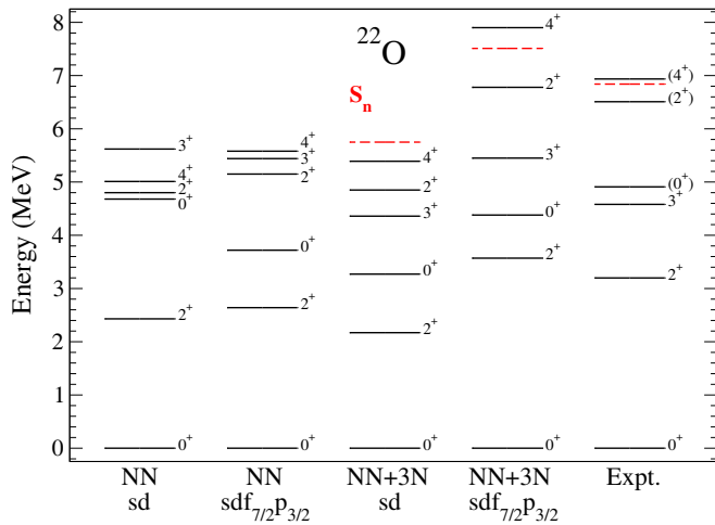
Fig. 3. Excitation energies of bound excited states in ^{22}\text{O} compared with experiment [4,5] (labels are as in fig. 2).
