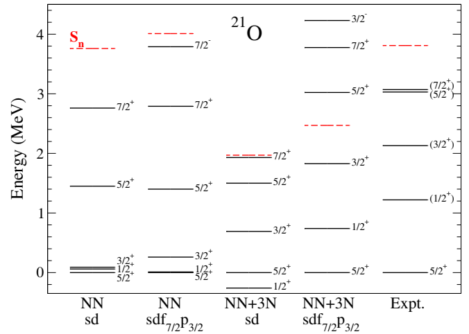
Fig. 2. Excitation energies of bound excited states in ^{21}\text{O} compared with experiment [4, 10]. The NN-only results are calculated in the sd and sdf_{7/2}p_{3/2} shells with empirical SPEs. The NN+3N energies are obtained in the same spaces, but with calculated MBPT SPEs, including 3N contributions to valence two-body interactions and SPEs. The dashed lines give the one-neutron separation energy S_n .
