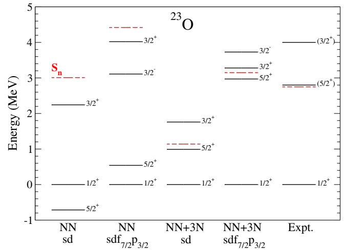
Fig. 4. Excitation energies of bound excited states in ^{23}\text{O} compared with experiment [7,8] (labels are as in fig. 2).
