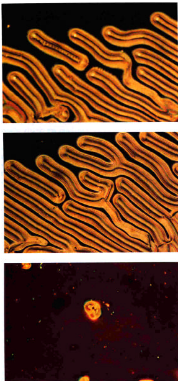
Figure 1. (a) (top) Cholesteric fingerprint texture observed for 4'-(pentyloxy)-4-biphenylcarbonitrile doped with P-trans-2 after irradiation with 435 nm light. (b) (middle) Cholesteric fingerprint texture observed for 3 doped with P-trans-2 after irradiation with 365 nm light. (c) (bottom) Compensated nematic structure obtained after irradiation at 313 nm for 20 min of a cholesteric thin film of 3 doped with 1 wt % of P-trans-2 . Viewed at ca. 150 \times magnification through crossed polarizers (reproduced at 50% of original size).
