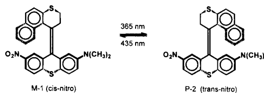
Scheme 1. Photoisomerization of M-1 and P-2
