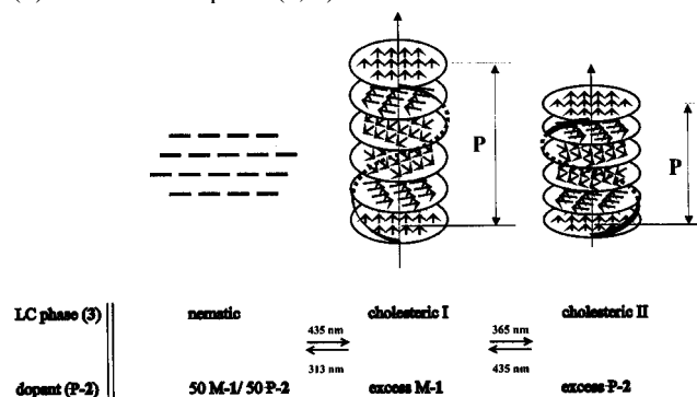
Scheme 2. Photochemical Switching Processes of LC-Phase ( 3 ) and Chiral Dopants ( 1 , 2 ) a
