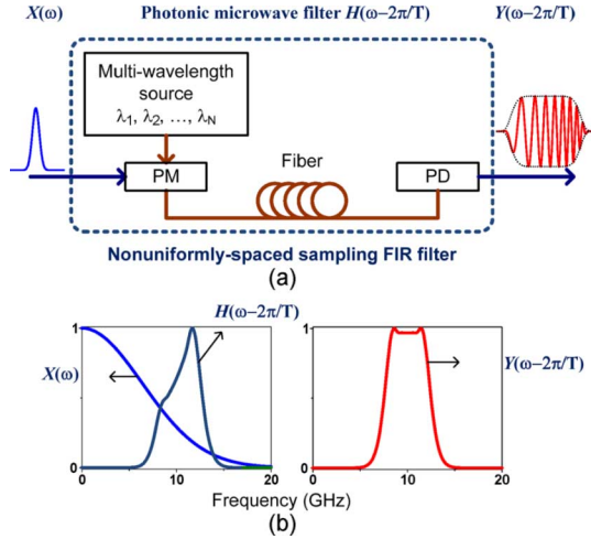
Fig. 1. (a) System setup. (b) Principle of the proposed technique for chirped microwave pulse generation.
