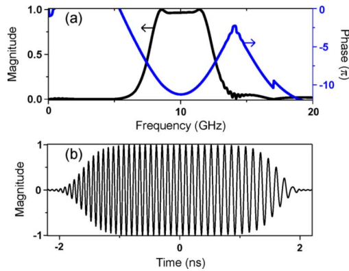
Fig. 3. (a) Spectrum of the chirped microwave pulse and (b) temporal waveform of the pulse.
