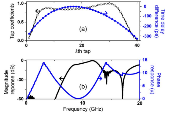
Fig. 2. (a) Filter design for the chirped microwave pulse generation. \square -line: the tap coefficient profile. \bullet -line: time delay differences. (b) Magnitude and phase responses of the filter.
