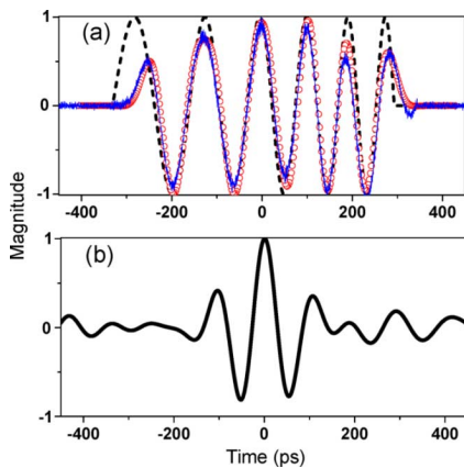
Fig. 4. (a) Solid line: the generated chirped microwave pulse. Dashed line: the desired chirped microwave pulse. Circle-line: Simulation result. (b) Correlation between the measured and the reference pulses.
