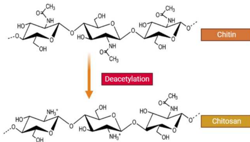
FIGURE 1 | Structure of chitin and chitosan. CH is a naturally occurring water-soluble cationic polysaccharide that is generated by alkaline deacetylation of chitin. CH is a linear polysaccharide composed of \beta -(1-4) linked 2-acetamide-2-deoxy-D-glucose (a neutral sugar unit GlcNAc or A-unit) and 2-amino 2-deoxy-D-glucose (a cationic sugar unit GlcN or D-unit). CH can have a broad range of degree of deacetylation ( F_A ), as well as variable chain length and molecular weight.
