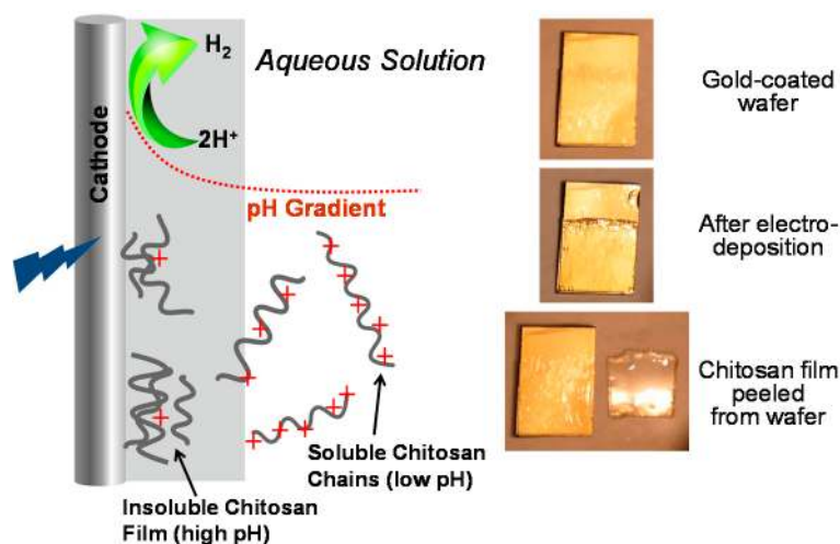
Figure 3. Chitosan’s cathodic electrodeposition. Cathodic reactions generate the localized high pH adjacent to the electrode that neutralize chitosan and trigger its sol–gel transition.
