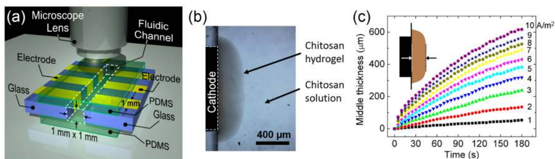
Figure 5. Cathodic electrodeposition allows control of chitosan film thickness. (a) Fabricated fluidic device used for in situ observation of chitosan's electrodeposition. (b) Photograph of a chitosan film electrodeposited onto the sidewall electrode address. (c) In situ measurements of chitosan's film thickness as a function of time and current density. Reproduced with permission from [77,78], published by Royal Society of Chemistry, 2010 and 2011.
