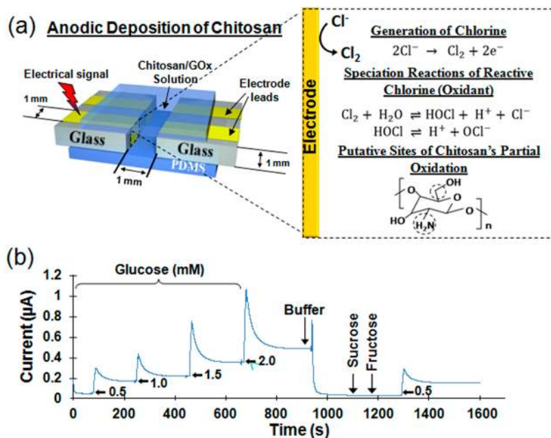
Figure 11. Anodic deposition of chitosan results from a sequence of chemical reactions that results in a covalently crosslinked network and possibly with covalently conjugated proteins. (a) Proposed deposition mechanism; (b) Results with the model biosensing enzyme glucose oxidase (GOx). Reproduced with permission from [131], published by American Chemical Society, 2012.
