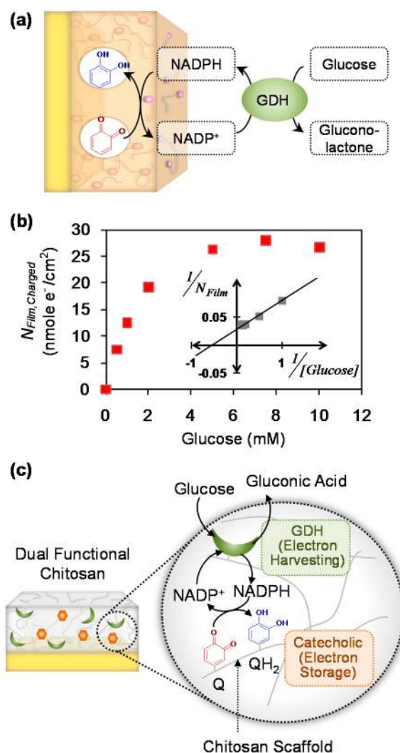
Figure 16. (a) Glucose dehydrogenase (GDH) catalyzed redox-cycling to charge the catechol-chitosan film; (b) Enzymatic charging is controlled by the electron source glucose (insert shows analogous Lineweaver-Burke plot); (c) Schematic illustrating how GDH harvests electrons from glucose and NADPH shuttles them to the grafted catecholic moieties where the electrons are stored. Reproduced with permission from [239] and [232], published by John Wiley and Sons, 2012 and Institute of Physics Publishing, 2013.
