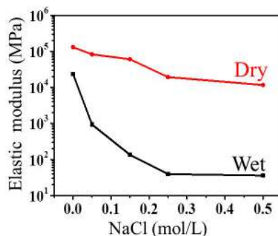
Figure 7. The properties of electrodeposited chitosan films are sensitive to the conditions used during the deposition process ( i.e. , the addition of salt to the deposition solution). The elastic modulus was measured by quartz crystal microbalance with dissipation. Reproduced with permission from [83], published by Royal Society of Chemistry, 2013.
