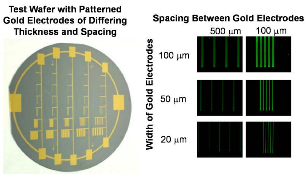
Figure 4. Spatial control of chitosan's electrodeposition. Chitosan was deposited onto gold electrodes that had been patterned onto a silicon wafer. The test wafer was designed to have electrodes of varying width and spacing. After deposition, chitosan was fluorescently labeled to facilitate visualization. Reproduced with permission from [75], published by American Chemical Society, 2003.
