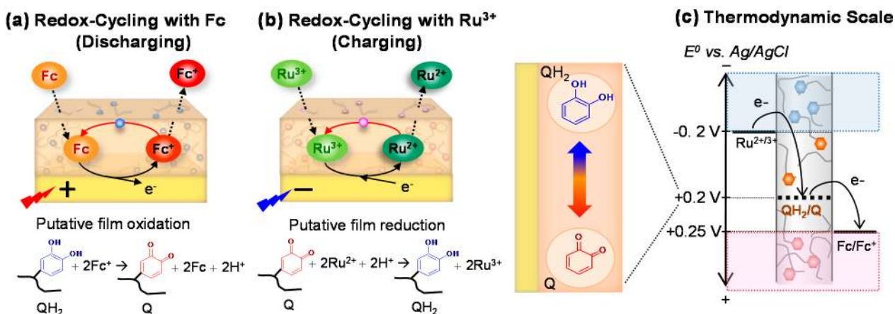
Figure 15. Redox-cycling of the catechol-chitosan redox-capacitor. (a) Oxidative redox-cycling can discharge electrons from the film; (b) Reductive redox-cycling can charge the films with electrons; (c) Thermodynamics controls the direction of electron transfer such that a mediator can only transfer electrons to/from the film in one direction. Reproduced with permission from [233], published by Royal Society of Chemistry, 2014.
