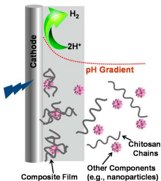
Figure 9. Co-deposition allows various biological and non-biological components to be assembled with and entrapped in the electrodeposited chitosan film.
