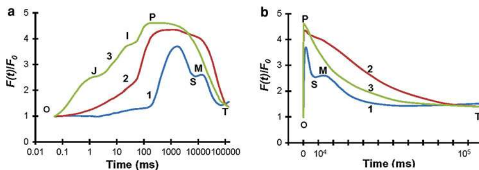
Fig. 2 Chlorophyll a fluorescence induction transients from a pea leaf (kept in darkness for 20 min before the measurement). They are plotted on a logarithmic time scale ( a ); and on a linear time scale ( b ). Wavelength of excitation: 650 nm. Excitation light intensity, at the
