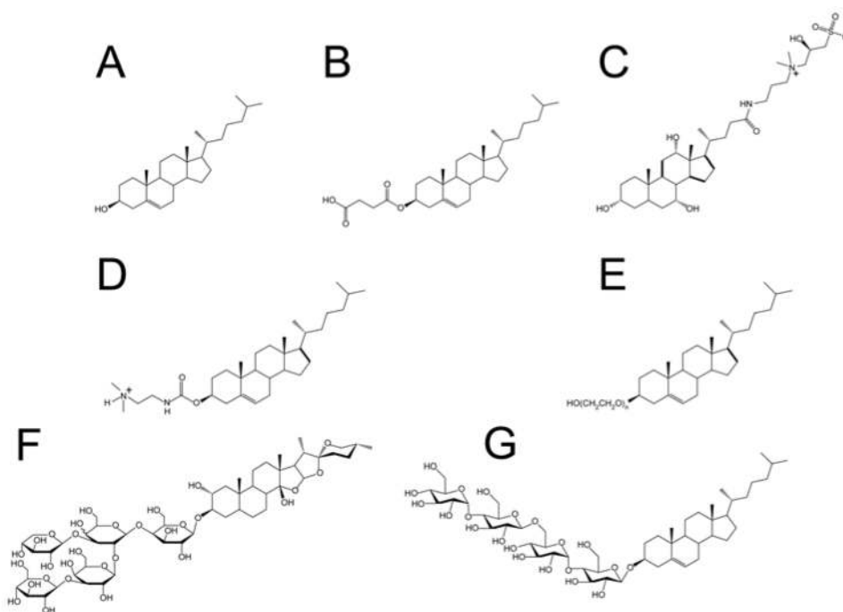
Figure 1. Structures of cholesterol-derived amphiphiles and related compounds: A. Cholesterol B. Cholesteryl Hemisuccinate (CHS) C. CHAPSO D. DC-CHOL (TMAEC-CHOL) E. Cholesteryl-PEG 600 (n average 10–11) F. Digitonin G. CHOBIMALT
