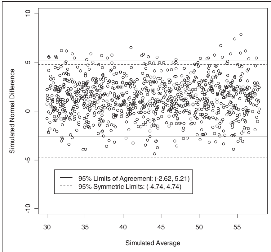
Figure 1. Bland and Altman plot from simulated 1000 normal differences and 1000 uniform averages.
