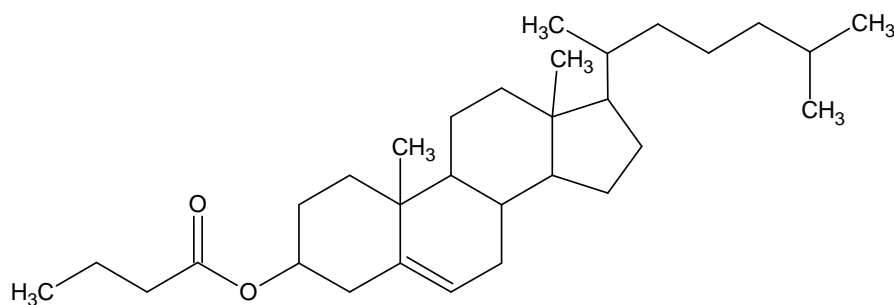
Figure 1. Structure of Cholesterylbutyrate.
