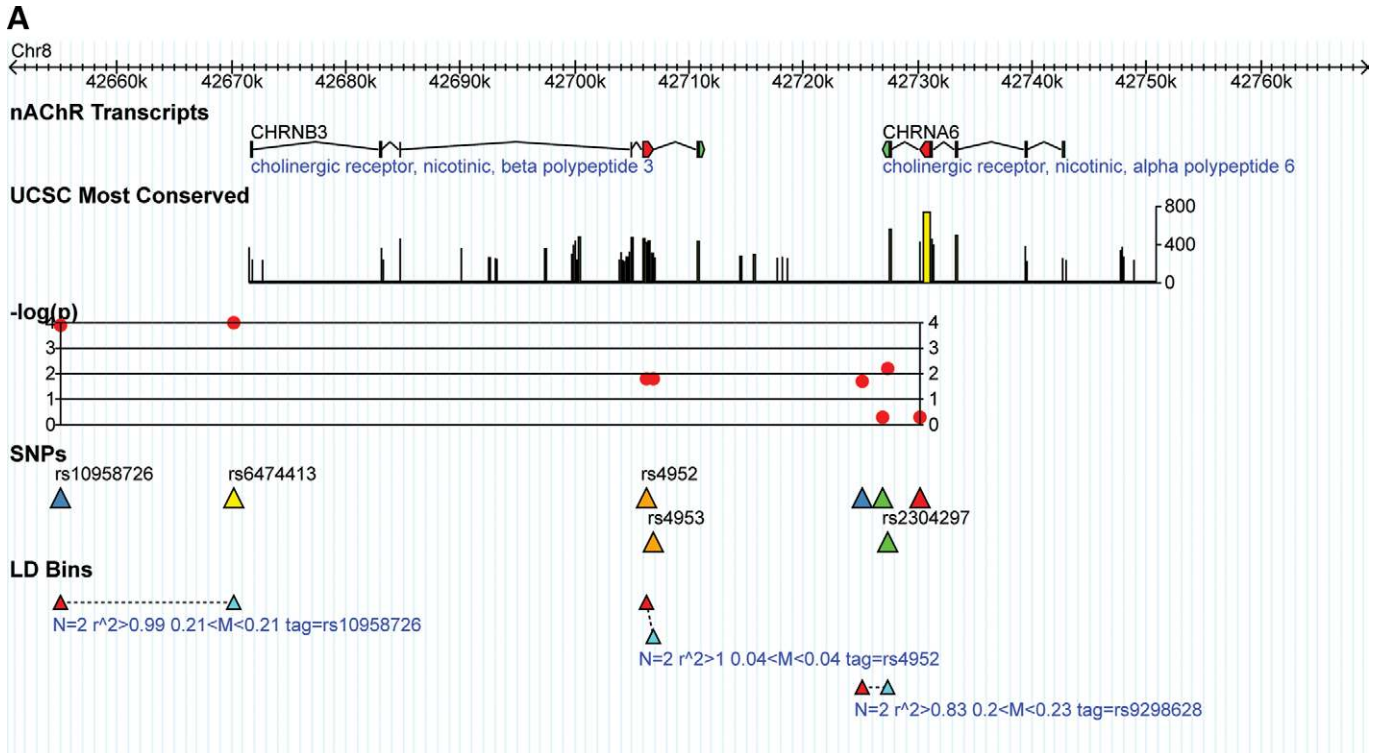
Figure 2. Detailed results for the top association signals. (A) The top two signals are near the CHRN3 nicotinic receptor gene on chromosome 8. (B) The Non-synonymous SNP rs16969968 and the CHRNA5-CHRNA3-CHRN4 cluster of nicotinic receptor genes on chromosome 15. SNPs that appear in Table 2 are labeled with dbSNP rs IDs. The track 'UCSC Most Conserved' ( http://genome.ucsc.edu , May 2004 build, table 'phastConsElements17way') highlights regions conserved between human and other species including the mouse, rat and chicken; the maximum conservation score is 1000. Primary P -values are plotted in red using the -\log(P) transformation. The 'LD Bins' track displays the distribution of SNPs from the 'SNPs' track into LD bins where all SNPs have r^2 \geq 0.8 in both cases and controls with the tag SNP. Only bins with more than two SNPs are shown, and bins are annotated with number of SNPs N , the minimum r^2 of the tag with the other SNPs in the bin, the range of allele frequencies in the bin and the tag SNP. (C) A legend indicating the color scheme.
