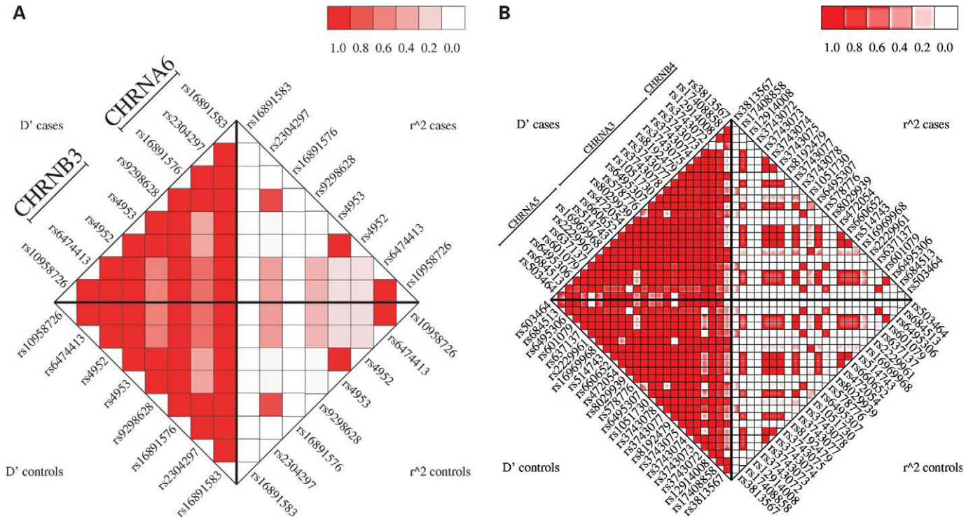
Figure 3. LD between markers in (A) the CHRN3-CHRNA6 and (B) CHRNA5-CHRNA3-CHRN4 clusters of nicotinic receptor genes.
