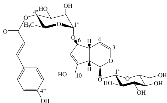
Lasianthoside I (3)
