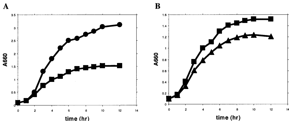
FIG. 3. (A) Growth of wild-type P. putida KT2440 in LB medium with (■) or without (●) 400 μM Cr(VI). (B) Growth of wild-type P. putida KT2440 (■) and the CRK4 mutant (▲) in LB medium with 400 μM Cr(VI). The data are the mean points of three independent measurements; the standard error of the mean was <7%.
