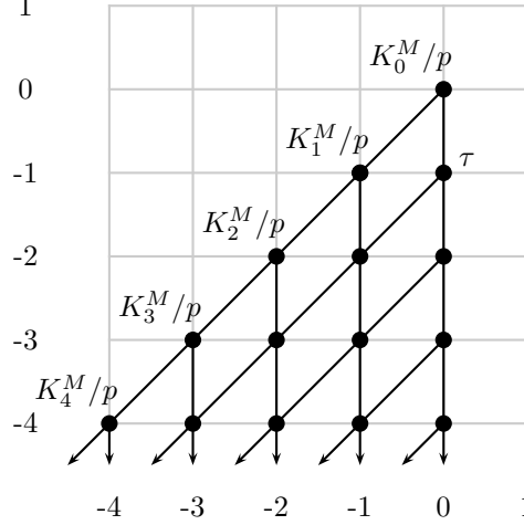
FIGURE 1. The cohomology of a point. The grading is homological to align with later homotopy group calculations. The topological degree is on the x -axis, and the motivic weight is on the y -axis. Each dot in column -n represents a copy of K_n^M(k)/p . Vertical lines indicate multiplication by \tau . Diagonal lines connect the source and target of multiplications by elements of K_1^M(k)/p .
