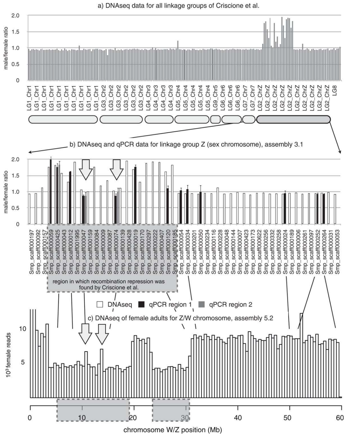
Figure 1 Next generation sequencing hit-count ratios between male and female genomes. (a) All scaffolds arranged by Criscione et al. [22] in linkage groups. For autosomes, the expected ratio would be 1; for Z-specific scaffolds, the expected ratio would be 2. Scaffolds are in the order defined by Criscione et al. (b) Male/female hit-count ratios and qPCR ratios for the Criscione et al. linkage group 2 (sex chromosomes). (c) Profile of hit counts along the latest version of the sex chromosome [21] for DNA extracted from females. One bar corresponds to 0.5 Mb. Arrows indicate the two pseudoautosomal blocks within the region where recombination is repressed.
