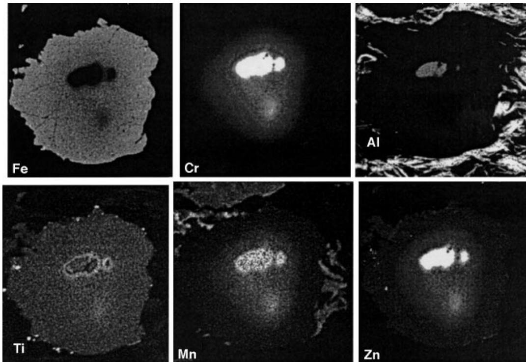
Fig. 15. X-ray intensity map of type 2 chromite with advanced magnetite replacement, Windarra. Field of view 0.5 mm. Strong zoning of Cr and Fe in magnetite, and ring of high Ti corresponding to innermost edge of magnetite rim, should be noted.
