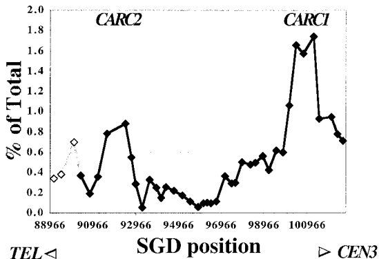
Figure 3. High resolution analysis of Mcd1p-binding sites on a region of chromosome III arm. (A) Physical Map of a region of the left arm of chromosome III, including LEU2 and other ORFs. Part of a full Ty2 retrotransposon inserted to the left of the LEU2 gene is shaded in gray. (B) Binding profile of Mcd1p on chromosome III arm. The amount of immunoprecipitated DNA (as percent of total) is plotted on the y axis versus DNA sequence coordinates on the x axis. The DNA sequence coordinates are aligned to the physical map in A. Gray shaded data points and line correspond to repetitive fragments within the Ty element.
