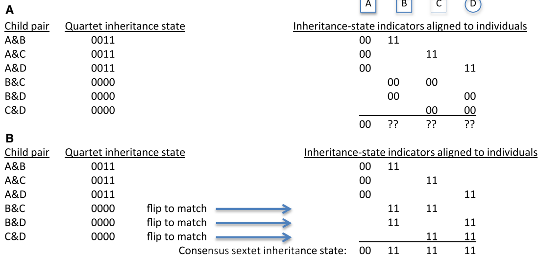
Figure 2. Constructing a Higher-Dimensional Inheritance State from Tiled Quartet States
