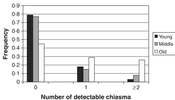
Fig. 1. Frequency of detectable chiasma on MI non-disjoined Ch 21 among women of different age groups having DS babies.
