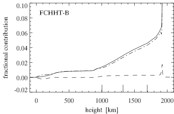
Fig. 12. Fractional collisional contribution \varepsilon_{\nu_0}[B_{\nu_0}(T) - \bar{J}_{\nu_0}]/S_{\nu_0}^l (dashed) and detour contribution \eta_{\nu_0}[B_{\nu_0}(T_d) - \bar{J}_{\nu_0}]/S_{\nu_0}^l (dot-dashed) to the H\alpha line source function. Their sum (solid) represents (S_{\nu_0}^l - \bar{J}_{\nu_0})/S_{\nu_0}^l . The ticks on the x -axis are at \tau_{\nu_0} = 3, 1, 0.3 in H\alpha .
