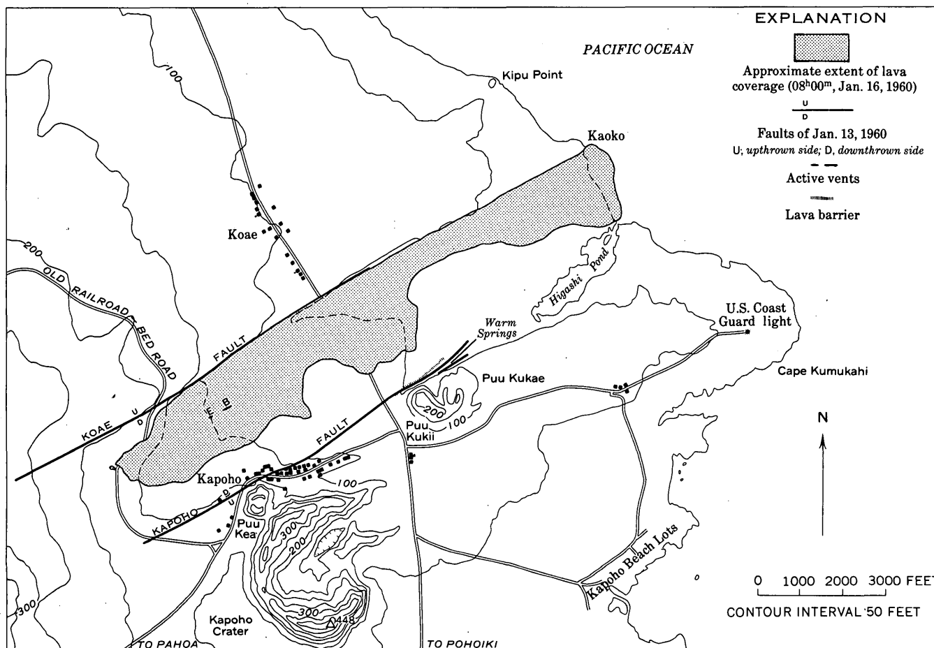
FIGURE 49.—Map of eruption area at 08 h 00 m , January 16, 1960.
