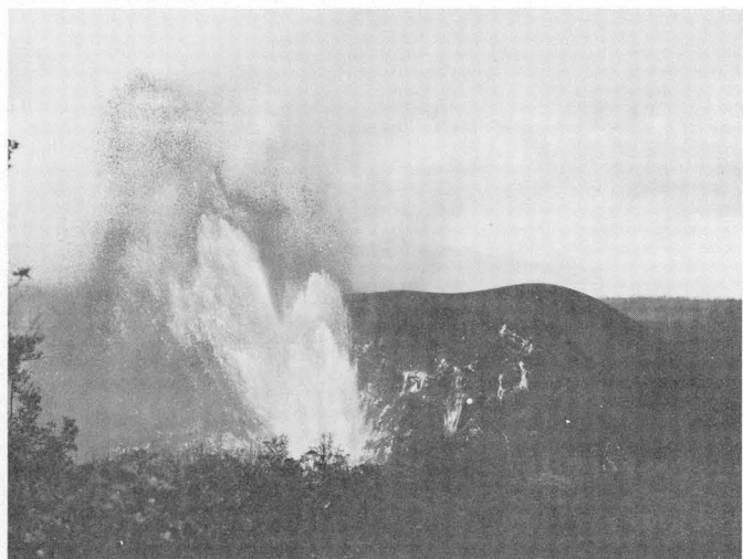
FIGURE 17.—November 29, 1959, 08 h 00 m . View from trail leading down to Byron Ledge showing the reduced fountain deflected northward by a collapse of the inner part of the cone. Note the new cone developing on the left shoulder of the old main cone (immediately to the right of the fountain).
