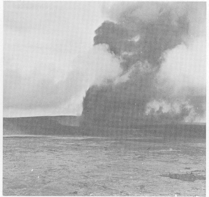
FIGURE 35.—December 17, 1959, 14 h 05 m . The 1,900-foot-high fountain as seen from the U.S. Geological Survey's Hawaiian Volcano Observatory. Top of fountain is inside the pushed-up cloud bank, and tremendous quantities of pumice rain out of the dark cloud on the right of the fountain.
