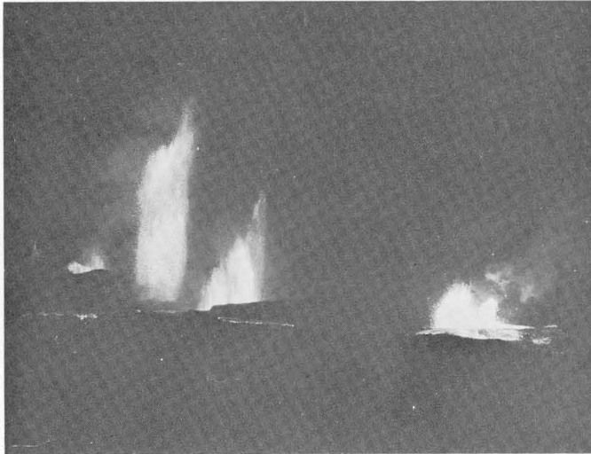
FIGURE 61.—January 28, 1960, 02 h 40 m . Renewed fountaining along the extended active rift, as seen from Puu Kukii. From left to right the active vents are: the spatter vent (E), main vent (B), and the two new vents, L and K.
