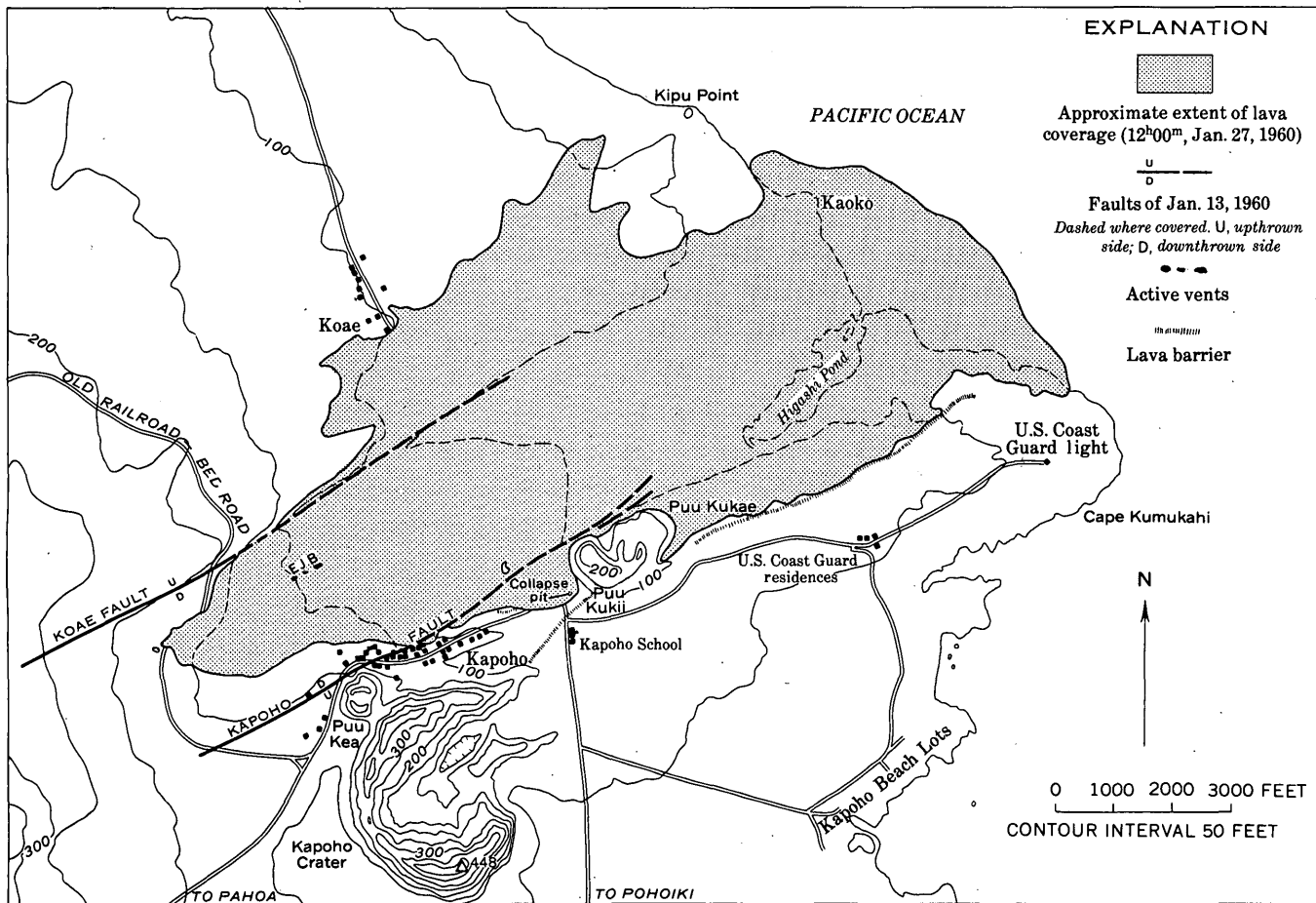
FIGURE 60.—Map of eruption area at 12 h 00 m , January 27, 1960.
