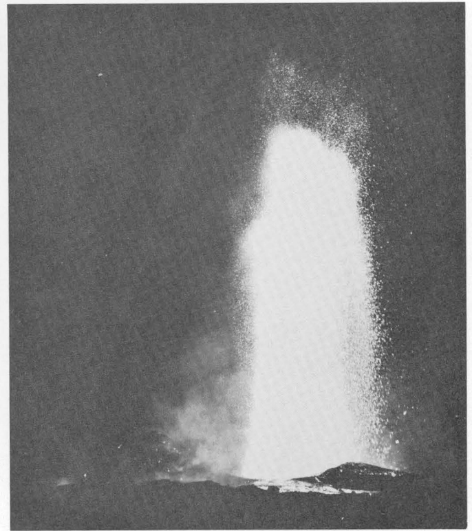
FIGURE 51.—January 18, 1960, 04 h 00 m . Main lava fountain, 1,600 feet high, as seen from top of Puu Kukii, 4,700 feet east of fountain.
