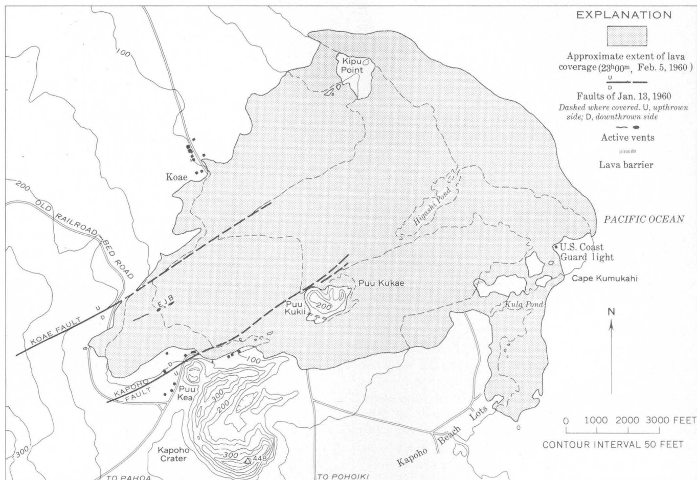
FIGURE 70.—Map of eruption area at 23 h 00 m , February 5, 1960.
