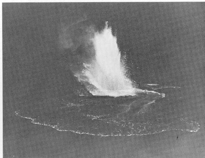
FIGURE 33.—December 17, 1959, 03 h 45 m . Fountain of the 14th phase, from Byron Ledge overlook, 17 minutes before activity ceased. The copious outpouring from the vent sweeps across the lake surface as one flow unit.
