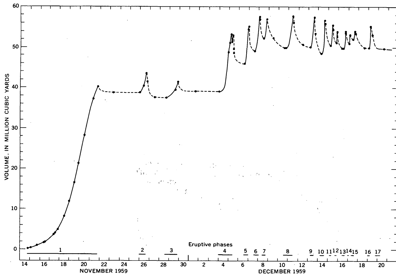
FIGURE 2.—Volume of lava erupted into Kilauea Iki during the 1959 summit eruption. Dashed line after the end of an eruptive phase represents backflow of lava down the vent. Each dot is a volume measurement.
