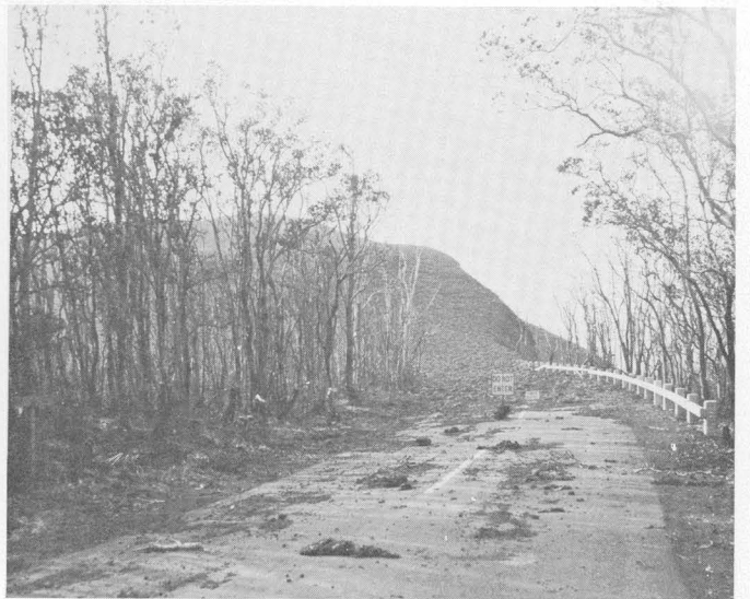
FIGURE 36.—December 17, 1959, afternoon. Cone and end of road west of Kilauea Iki overlook as seen immediately after the 1,900-foot-high fountain of the 15th phase. Note the large masses of spatter lying on road.
