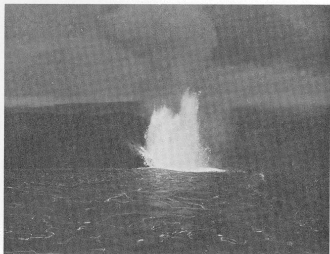
FIGURE 21.—December 5, 1959, 06 h 30 m . High, exceptionally level lava lake and relatively small fountain of the fourth phase just prior to the period of backflow concurrent with fountaining, as viewed from Byron Ledge overlook. Crust of lake is continually foundering and reforming.
