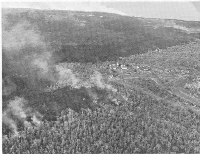
FIGURE 66.—February 1, 1960. Aerial view northeastward showing flows encircling the U.S. Coast Guard residence area. Flows have cut road leading to lighthouse out of picture on the right.
