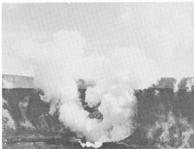
FIGURE 80.—March 11, 1960, 08 h 30 m . View northward of steam rising from third (northeast) collapse pit in floor of Halemaumau. Main caldera wall is in background.
