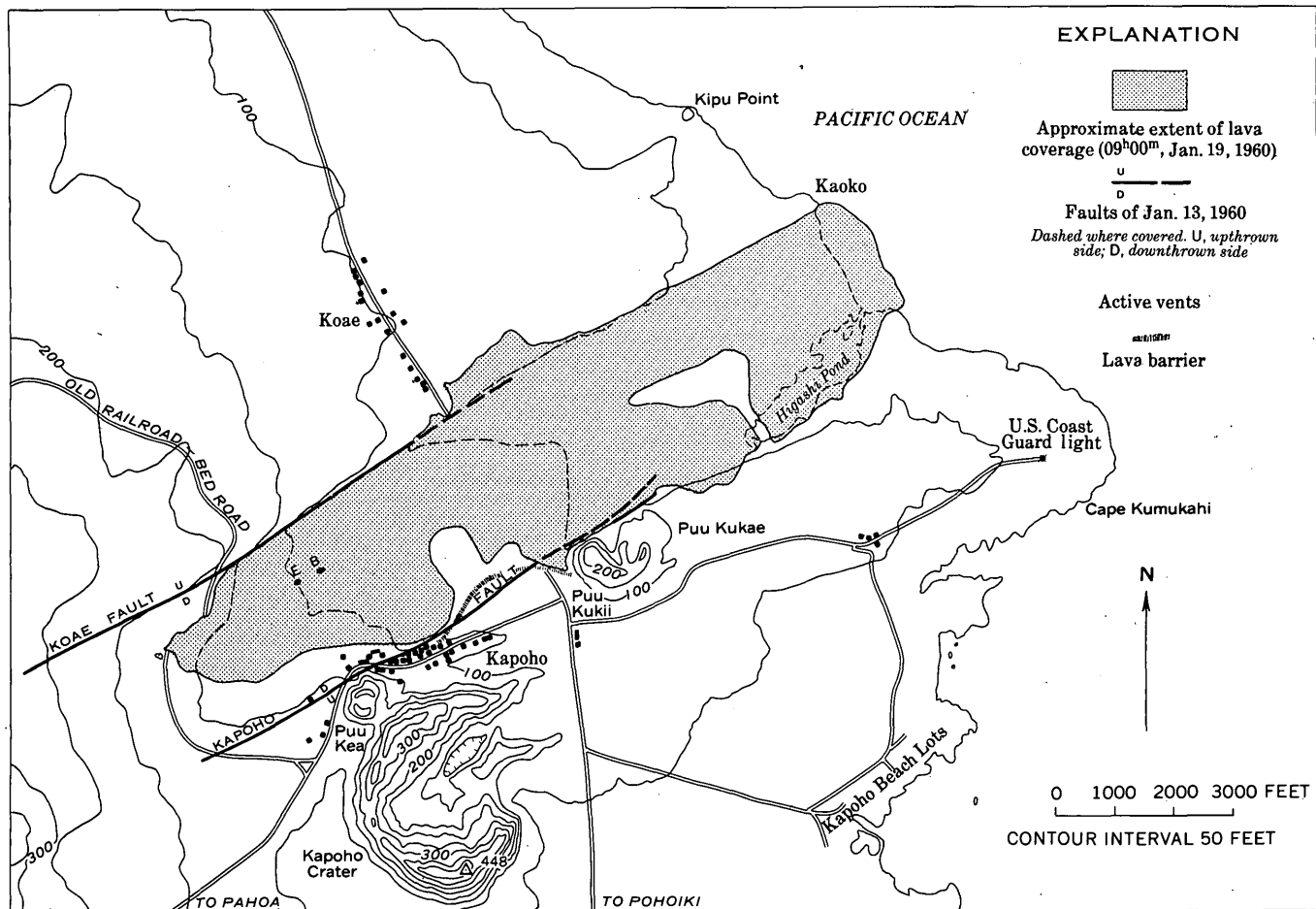
FIGURE 52.—Map of eruption area at 09 h 00 m , January 19, 1960.
