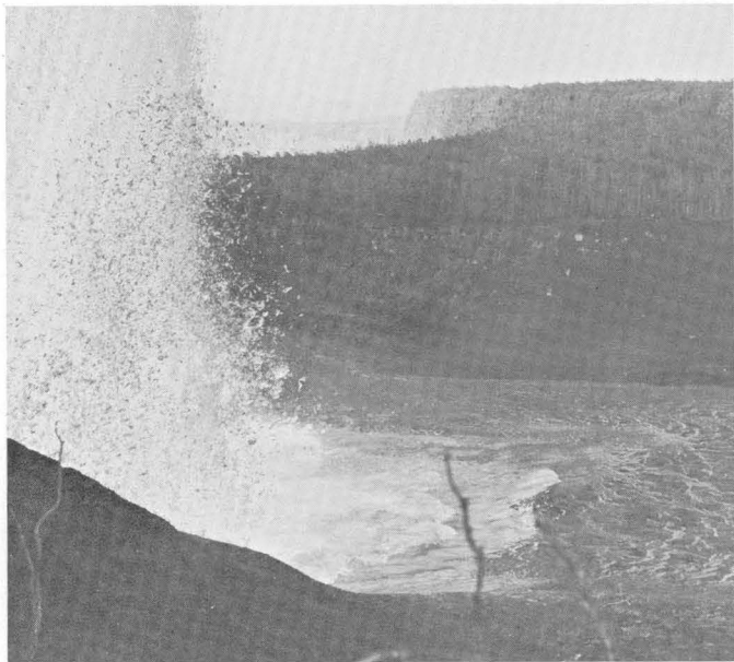
FIGURE 30.—December 14, 1959, 15 h 00 m . Fountain and lake from west end of Kilauea Iki overlook showing development of lava waves at base of fountain in high lava lake.
