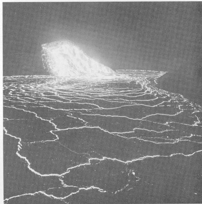
FIGURE 25.—End of the seventh phase of activity as seen from Byron Ledge overlook. Top : December 8, 1959. Fountain and lake a few minutes before activity stopped. Photograph by National Park Service. Bottom : December 8, 1959, about 20 h 12 m . Same view a few seconds after fountaining stopped. The cone is still aglow from incandescent spatter, and the lake crust is already fractured and moving as lava pours back down the vent. Photograph by National Park Service.
