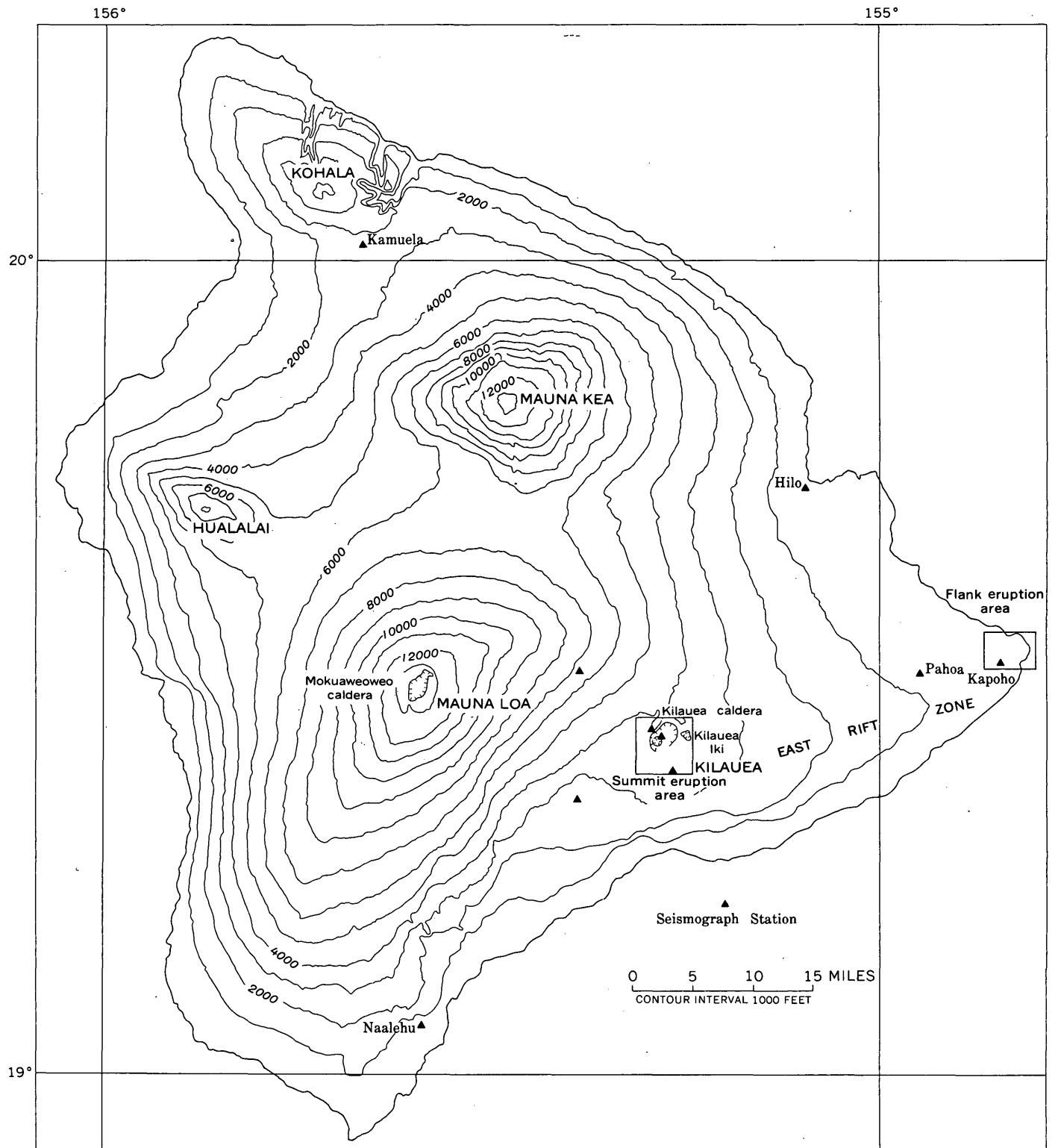
FIGURE 1.—Map of the Island of Hawaii showing summit and flank eruption areas on Kilauea and location of U.S. Geological Survey seismograph stations.
