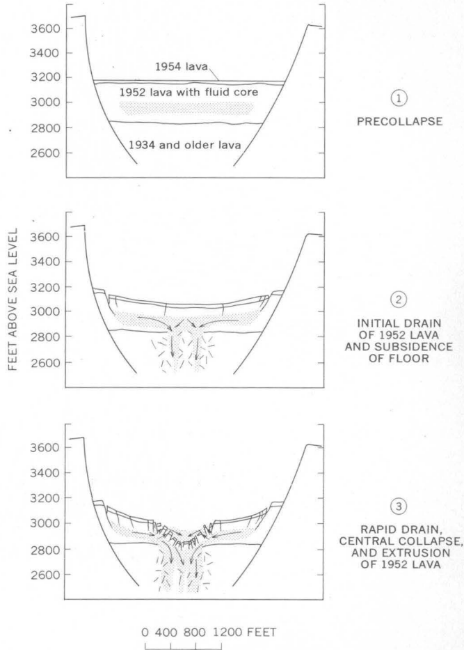
FIGURE 77.—Hypothetical east-west sections through Halemaumau showing development of principal collapse features.
