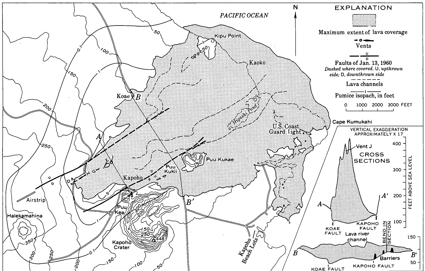
FIGURE 75.—Map and cross sections of the eruption area showing maximum extent of lava coverage and isopachs of the pumice blanket.
