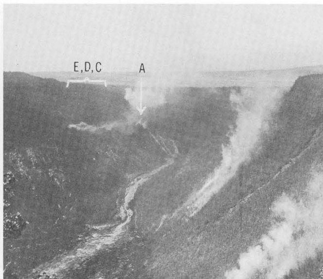
FIGURE 7.—November 15, 1959. View from Byron Ledge overlook showing the fountain at A, braided lava cascades down the crater wall to the lava river, the main cascade, and the lava lake. Fume rises from the activity at A and from the dead vents at C, D, and E. On the north wall of the crater a number of forest fires sweep up the slope. Photograph by National Park Service.
