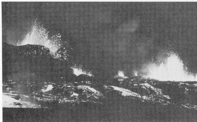
FIGURE 71.—February 5, 1960, 22 h 30 m . Renewed outbreak west of the spatter cone (left) along original fissure. Very fluid lava pours northward toward the old railroad-bed road.
