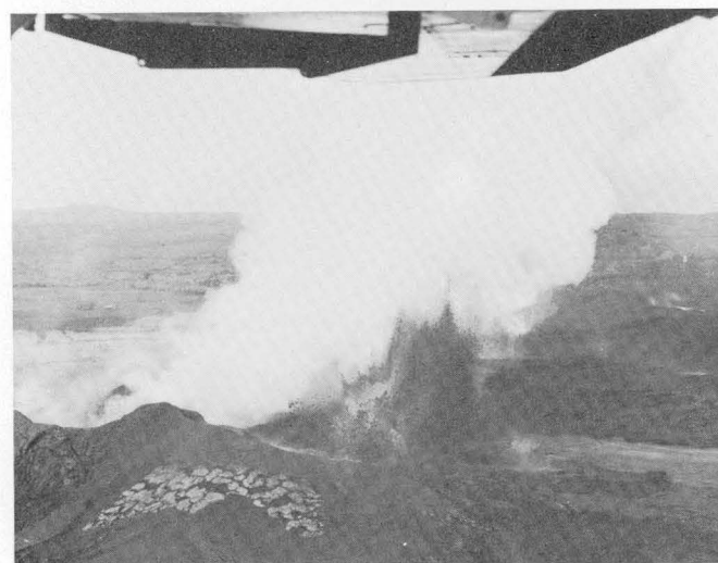
FIGURE 68.—Fountains and cone. Top : February 2, 1960. View northeastward from old railroad-bed road. Large fountain plays from vent L. Small fountain from main vent is barely visible above rim of cone, and spatter vent emits copious fume. Bottom : February 2, 1960. Aerial view northeastward showing large fountain playing from main vent (center) and the low boiling emission of lava from vent L (right). Note the patchwork pattern of congealed spatter on cone, formed by differential downslope movement.
