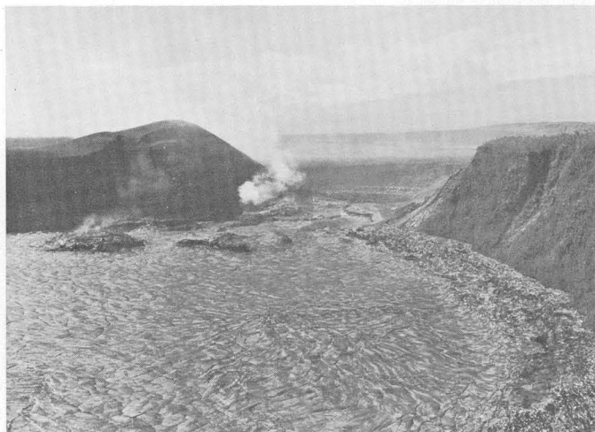
FIGURE 38.—December 20, 1959. View from Byron Ledge overlook after all activity ceased. The black ledge, 50 to 200 feet wide and approximately 50 feet high, surrounds the entire lake. Vent and largest island continue to emit fume. Compare with figure 7 taken on second day of eruption. Photograph by R. T. Haugen, National Park Service.
