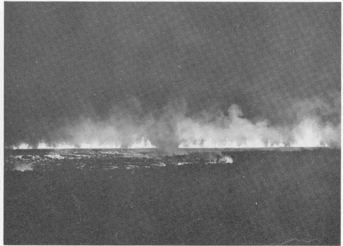
FIGURE 42.—January 13, 1960, 20 h 00 m . Initial outbreak of flank eruption. View northeast toward curtain of fire and first lava flows, half an hour after outbreak. Erupting fissure is about 3,000 feet long and lava fountains are 50 to 100 feet high.
