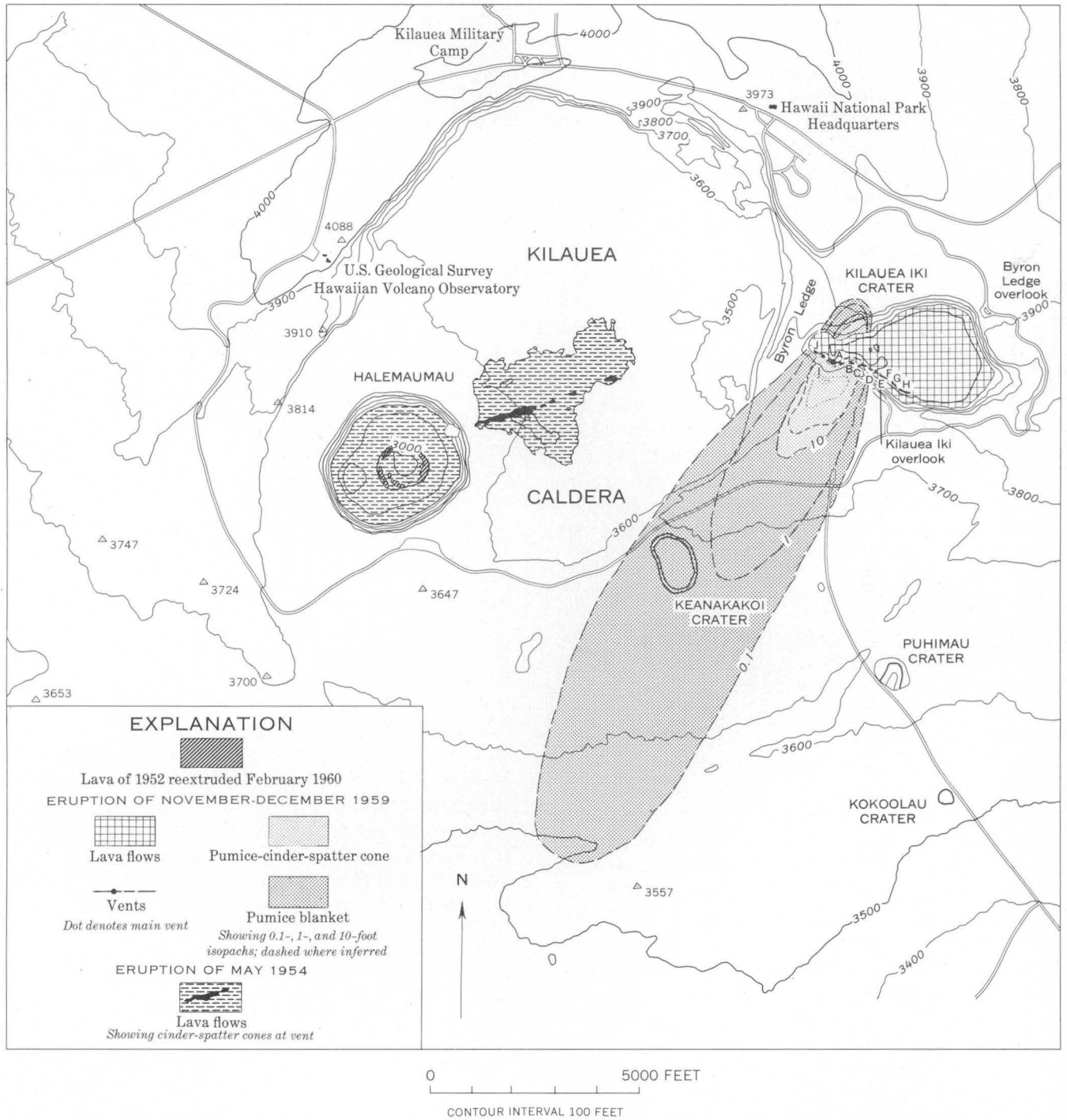
FIGURE 3.—Map of the Kilauea summit area showing principal 1959 eruptive features in and around Kilauea Iki and the 1960 collapse in Halemaumau. Location of outline and vents of the 1954 flow on the caldera floor is from Macdonald and Eaton (1957).
