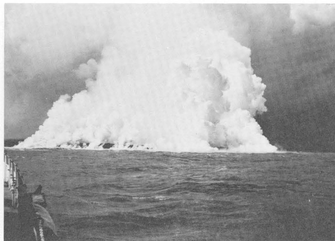
FIGURE 45.—January 15, 1960, 12 h 00 m . Early lava flow pouring into the ocean behind a massive curtain of steam. Vessel is approximately 1,000 feet east of the front. Photograph by R. T. Haugen, National Park Service.
