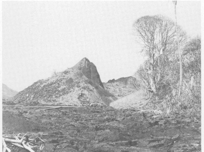
FIGURE 67.—Small fault blocks pushed upward and tilted by shallow intrusion of lava through old cinder cone (Puu Kukii) during the period January 28 through February 1. Photograph was taken March 23, 1960.
