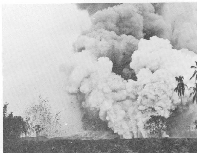
FIGURE 44.—Steam and ash production from the early vents. Top: January 14, 1960, 07 h 00 m . Violent steam emission caused by ground water rushing into the subsurface eruptive conduits. Darker steam cloud is choked with fine ash particles. Bottom: January 14, 1960, 10 h 00 m . Violent steam emission and adjacent moderate lava fountaining. Note the volcanic debris carried high into the steam cloud.
