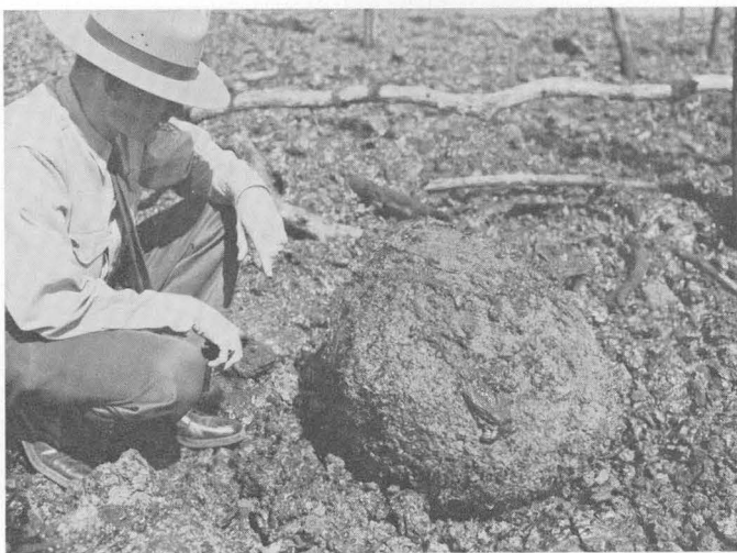
FIGURE 24.—Three-foot, spatter-encrusted, cored lava bomb photographed where it fell on the east side of the cone during the seventh phase of activity. Photograph by R. T. Haugen, National Park Service.
