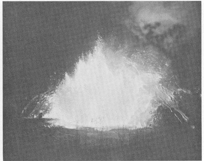
FIGURE 23.—December 7, 1959, 23 h 30 m . Low, broad fountain of the sixth phase and spatter-fed flows cascading down the flanks of the cone. Note the waves forming on the lake at the base of the fountain. View from north end of Byron Ledge. (See fig. 22 for contrast.)
