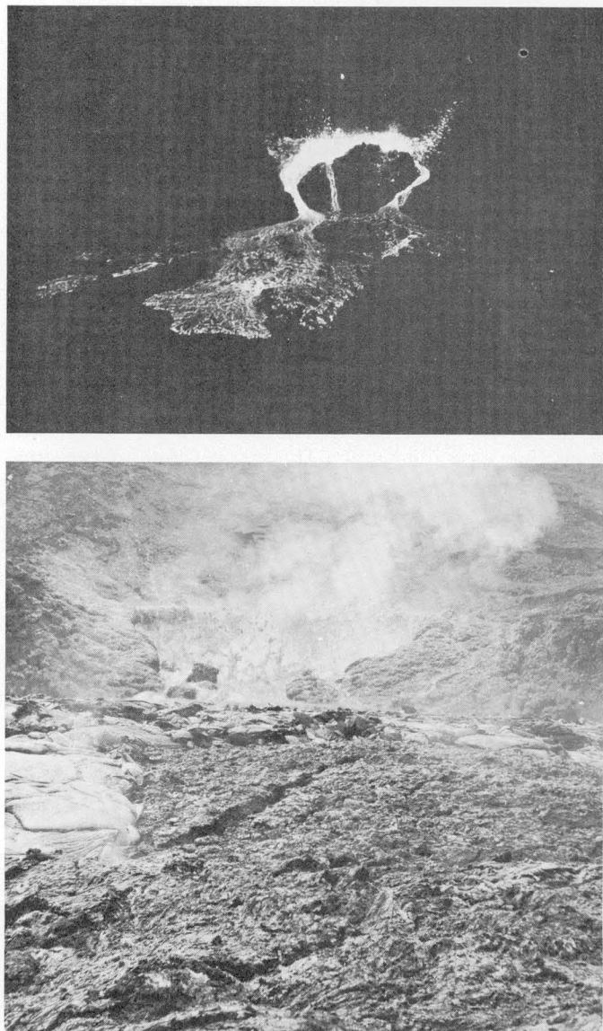
FIGURE 20.—Views of fourth-phase fountain and lava flows. Top : December 4, 1959, 06 h 00 m . Small fourth-phase fountains feed early flows on the lake surface 40 feet below the vent. View from crater rim opposite vent. Bottom : December 4, 1959, 12 h 00 m . Small spatter fountain plays in caldron over vent. Lava pours over breach in caldron and spreads across cooled third-phase lava in foreground.
