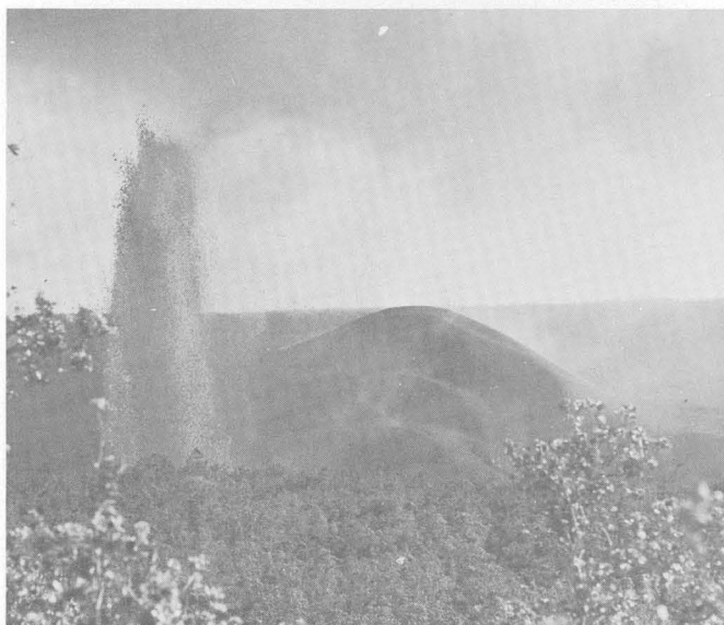
FIGURE 12.—November 20, 1959, early afternoon. Fountain and cone from the north end of Byron Ledge, showing prominent slump features along inner face of cone.
