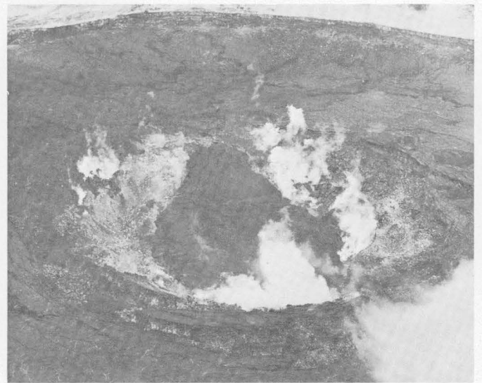
FIGURE 78.—Early collapse features in Halemaumau. Top : February 9, 1960. Aerial view northwestward across Halemaumau. Scarp encircling floor of crater marks outer limit of saucer-shaped subsidence. Steam rises from periphery of central collapse pit, partially filled with reextruded 1952 lava. Note wormlike pressure ridges crisscrossing floor. Diameter of central collapse pit is about 1,000 feet. Bottom : February 13, 1960. View of central collapse pit from south rim of Halemaumau. The small dark lava pond merges imperceptibly with the steep lava delta on far wall of pit.
