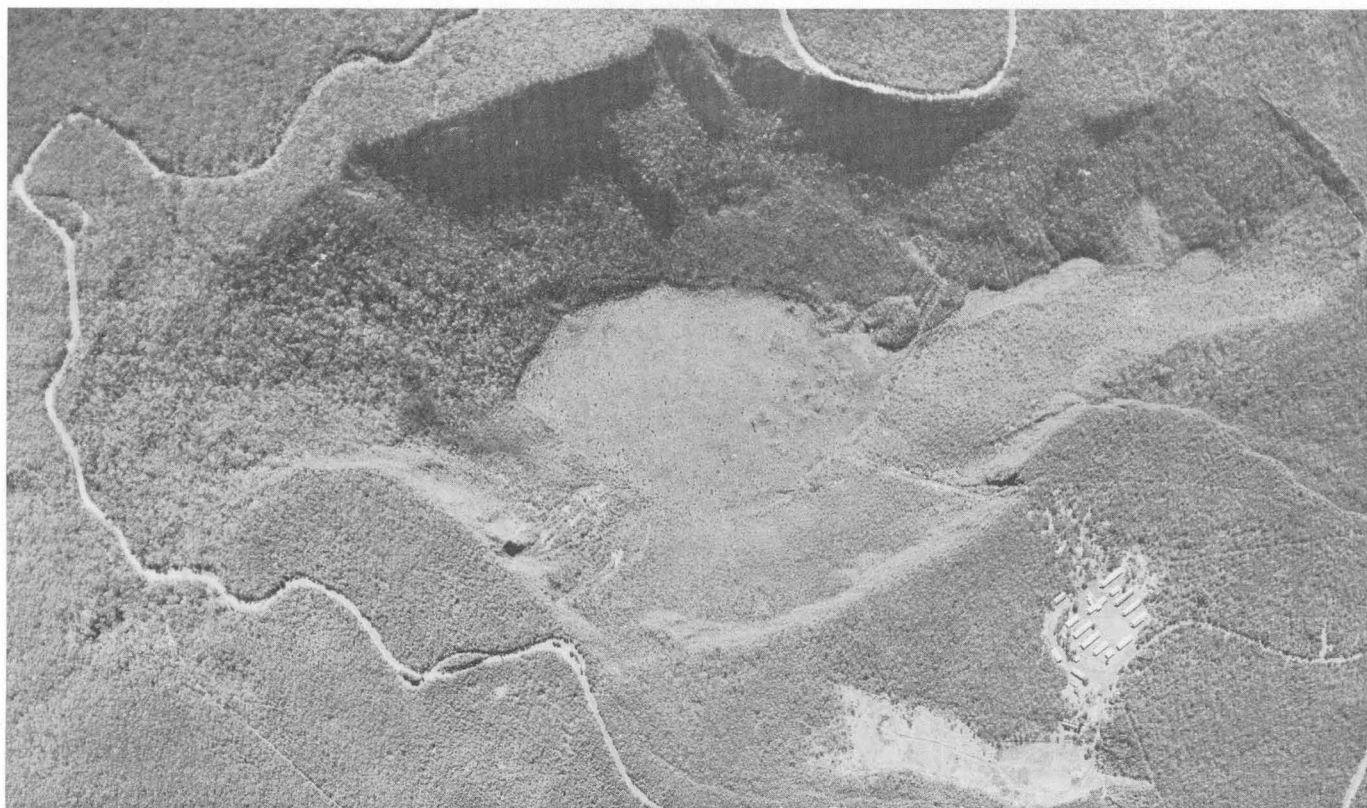
FIGURE 4 (above and right).—Aerial views of Kilauea Iki Crater before and after the 1959 summit eruption. The two principal overlooks into the crater, from which many of the pictures reproduced in this paper were taken, are labeled. Both photographs are approximately the same scale, but the one on the right shows considerable distortion. Above : U.S. Navy aerial photograph taken in 1948. The flat, ellip-
