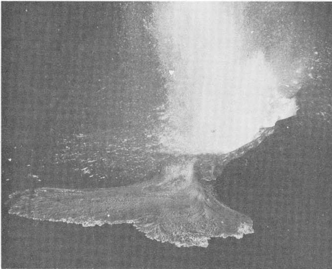
FIGURE 16.—November 28, 1959, 21 h 00 m . View from Byron Ledge showing small incandescent tongues of very fluid lava flowing into the west bay of the crater from the base of the fountain.
