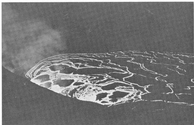
FIGURE 32.—December 15, 1959, 22 h 00 m . A wide stream of lava pours back into the vent half an hour after the end of 12th phase. Huge rafts of solid lake crust, continually breaking as the backflow stream converges near the vent, are mixed and swallowed with the returning lava. View from top of cone almost directly above vent.
