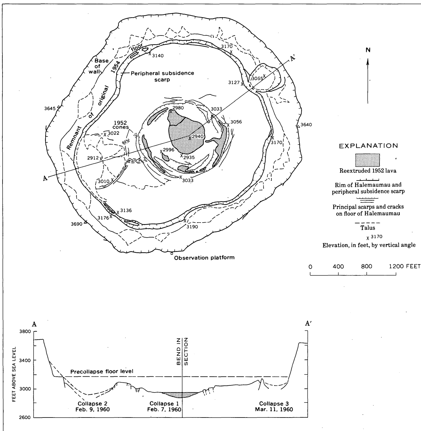
FIGURE 76.—Map and cross section of Halemaumau showing principal features of the 1960 collapse.
