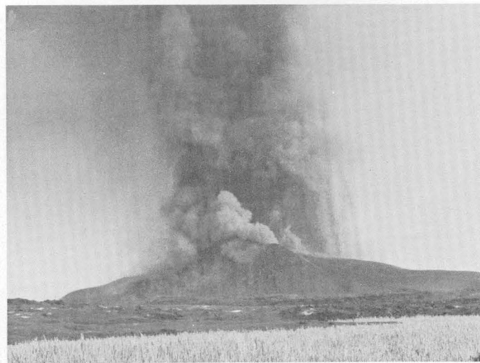
FIGURE 63.—Views of vent area. Top : January 29, 1960, 11 h 00 m . Cone and fountain viewed from the west. Small gushing fountain at base of spatter cone (vent E) bursts through shallow lava lake. Fountain from the main vent B in cinder-pumice cone behind spatter cone is about 600 feet high. Bottom : January 30, 1960. Heavy pumice fallout from main fountain covers top of fuming spatter cone. View is from the west. Compare with activity in top photograph.
