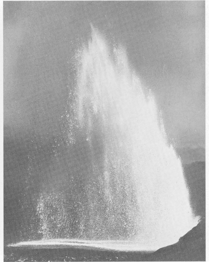
FIGURE 14.—November 21, 1959, 18 h 00 m . Northward-jetting fountain is blasting through the lake lava and debris is falling on the lake surface. View is from Byron Ledge.
