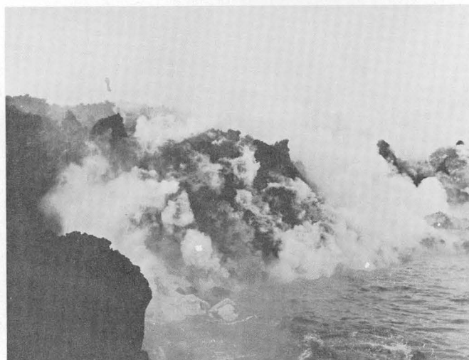
FIGURE 54.—Aa lava flow entering the ocean. Top : January 21, 1960. Heavy turbulent steam clouds rise from the front of a massive aa flow as it slowly pushes into the ocean. Small blasts of comminuted rock, which frequently exploded from the water, are not visible in the picture. Bottom : January 21, 1960. Closeup of same flow entering the ocean.
