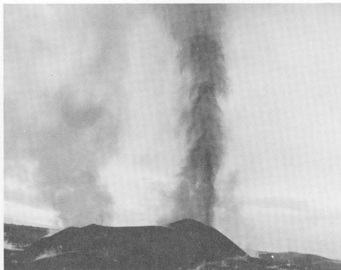
FIGURE 72.—February 16, 1960. Gas-cinder jet shooting to 1,000 feet from vent J as viewed from Puu Kea. Spatter vent E (left) emits strong fume cloud. Steam rising from flows and cone is from recent heavy rain.
