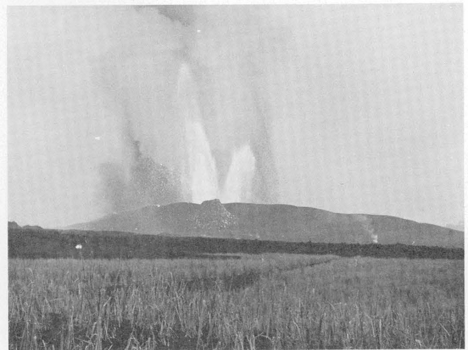
FIGURE 53.—Main lava fountain and cinder-pumice cone. Top : January 19, 1960. View eastward from old railroad bed road showing pumice from vent B pelting southwest flank of cone. Flows in sugar cane field in the foreground are from vents (out of picture on the left) that were active briefly along the curtain of fire on January 13, Bottom : January 22, 1960, 16 h 00 m . View eastward from old railroad bed road showing main V-shaped lava fountain (vent B) and small parasitic spatter cone (vent E). Large fountain apparently originating from the spatter cone is actually rising from the main vent beyond. Compare features with those above, taken from approximately the same location 3 days earlier.
