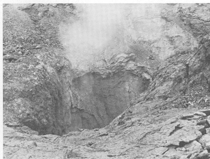
FIGURE 39.—Closeup views of vent. Top : December 22, 1959. Strong emanation of fume from vent, 2 days after cessation of activity. Lava flows in front of observer are from the 17th phase. Bottom : December 24, 1959. Slightly closer view showing only minor fume emission from the vent. Dense lava coating the wall of vent has already begun to spall off. Vent is 100 feet across greatest dimension.
