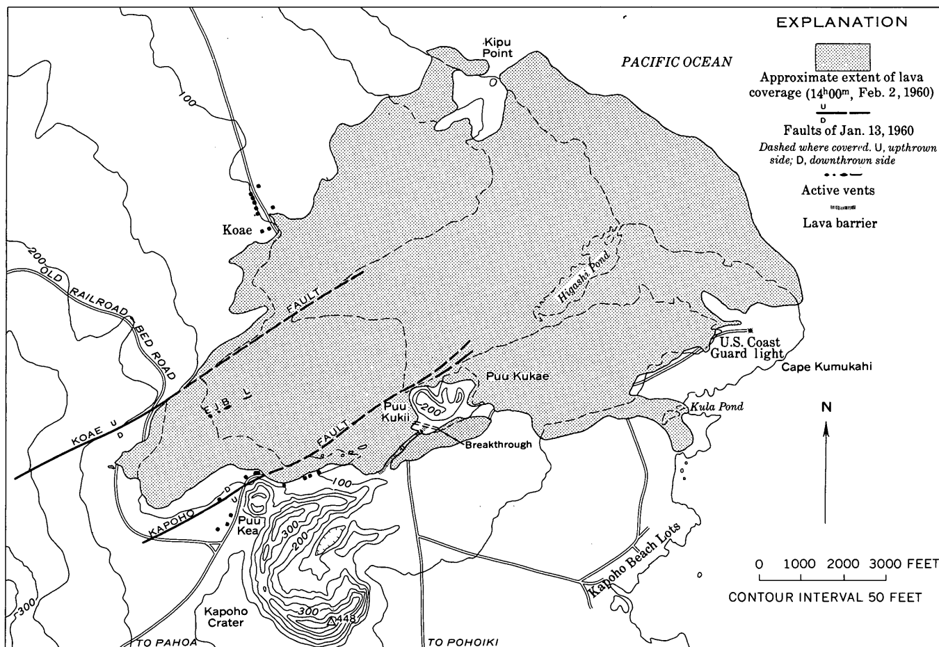
FIGURE 69.—Map of eruption area at 14 h 00 m , February 2, 1960.
