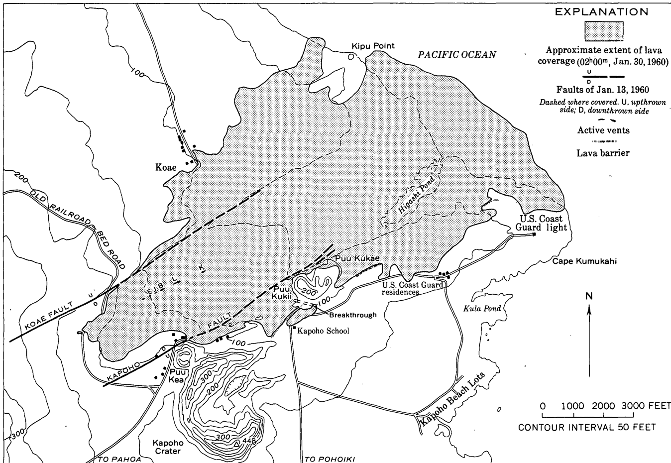
FIGURE 65.—Map of eruption area at 02 h 00 m , January 30, 1960.
