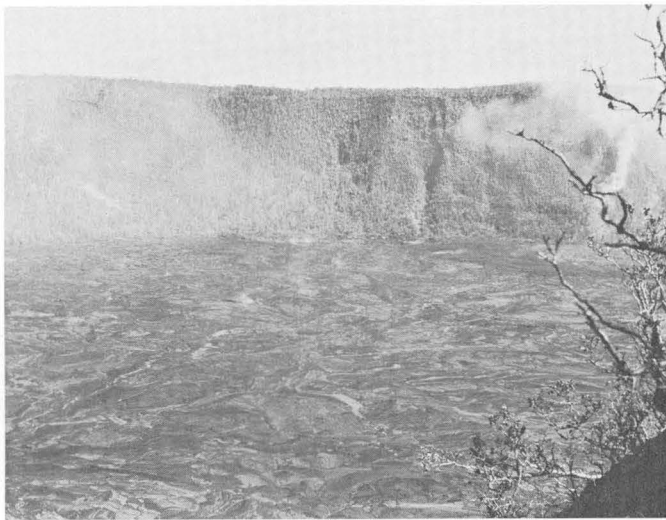
FIGURE 13.—Fountain and lake during the last day of the first phase, viewed from Kilauea Iki overlook. Top : November 21, 1959, 12 h 30 m . Relatively small fountain with ejecta falling directly upon the lake surface. Bottom : November 21, 1959, 13 h 00 m . Exceptionally level surface of the 330-foot-deep lava lake. Lighter areas and bands are fluid lava oozing and squeezing up around foundering plates of the crust on the continually reworked surface.
