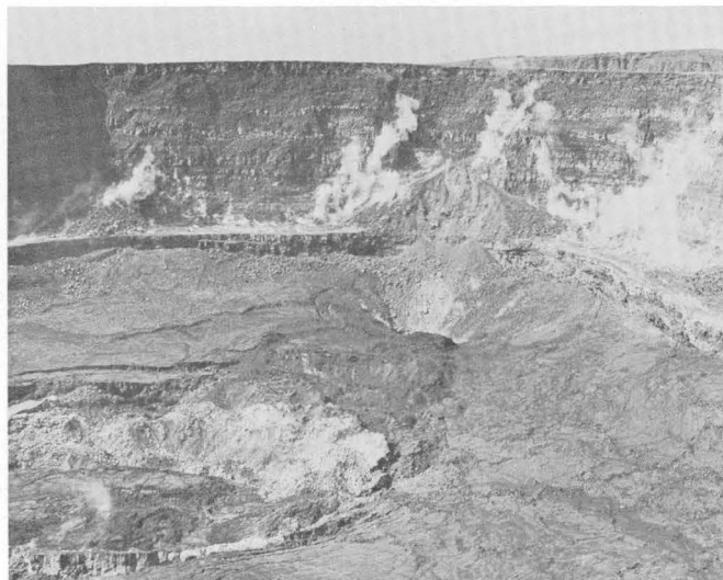
FIGURE 79.—View southward across Halemaumau showing saucer-shaped subsidence of floor, central collapse pit (left), and second (southwest) collapse pit at base of large talus pile in background.
