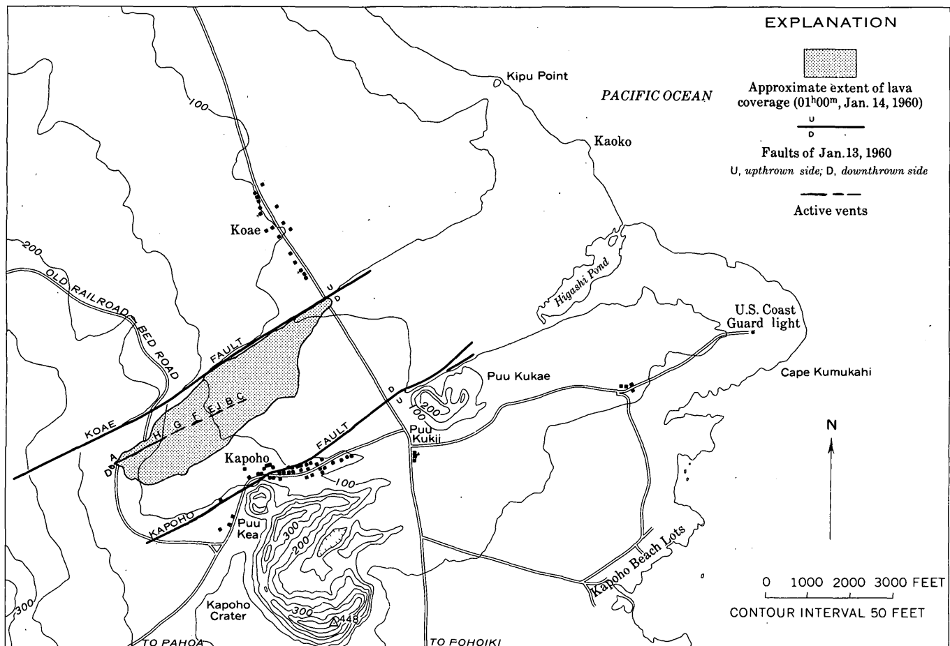
FIGURE 43.—Map of eruption area at 01 h 00 m , January 14, 1960.
