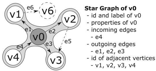
Fig. 13 Star Graph partitioning by example
