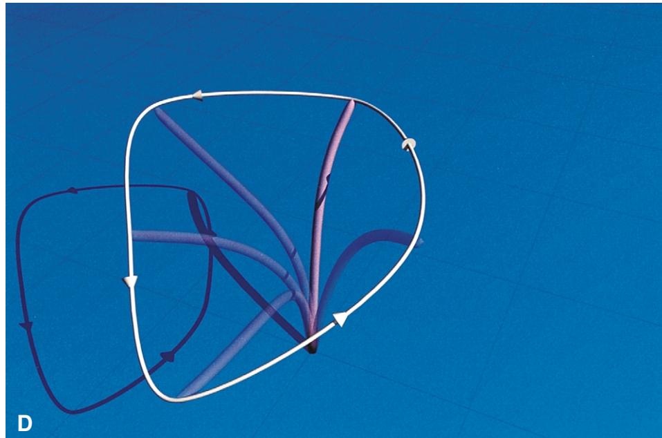
FIG 1. (continued) D , Diagram of the dyskinetic beat pattern observed for cilia with a transposition defect. Cilia beat in a large circular gyrating motion about the base of the cilium.
