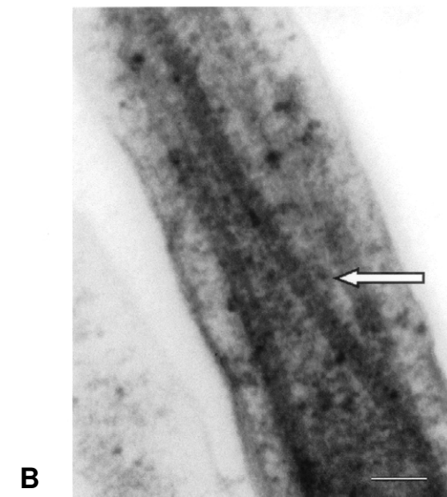
FIG 2. A, Electron micrograph of ciliary cross-section illustrating transposition defect. B, Electron micrograph of longitudinal section of ciliary axoneme illustrating the crossover of the peripheral microtubular doublet into the central position seen in the ciliary transposition defect.
