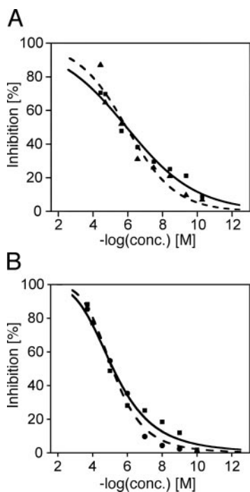
FIG. 3. Inhibitory activity of cinanserin and its hydrochloride on the proteolytic activity of SARS-CoV 3CL pro (A) and HCoV-229E 3CL pro (B). Inhibition of cleavage was measured by FRET using a peptide substrate labeled with a pair of fluorogenic dyes. Cinanserin, solid line (data points are shown as squares); cinanserin hydrochloride, dashed line (data points are shown as triangles or circles); conc., concentration.
