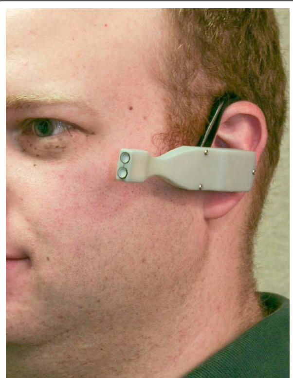
Figure 5 Close-up photograph of the Daysimeter. Two light sensors are located near the plane of the cornea, calibrated in terms of their absolute, spatial and spectral response to provide both photopic and circadian light readings. The rear housing attached to the earpiece contains accelerometers for measuring activity as well as memory and control circuitry, all powered by a coin-cell battery.
