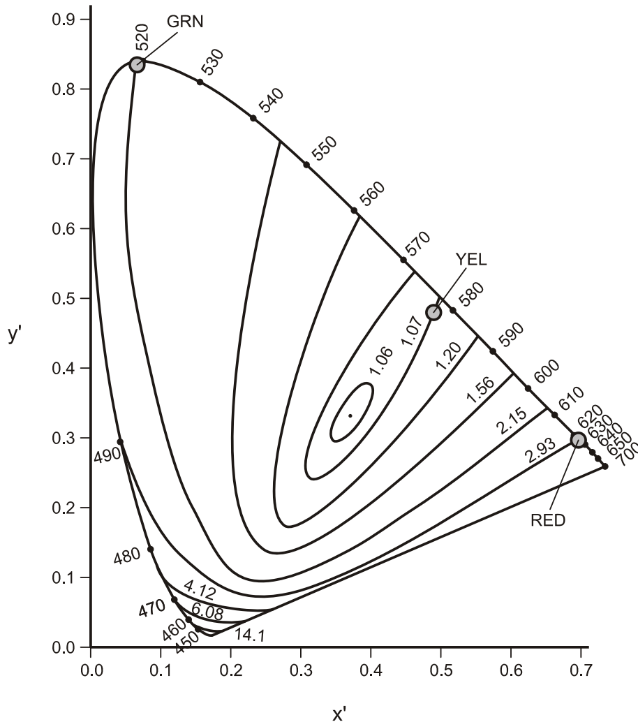
Figure 2 Chromaticity diagram based on the Judd correction [22], showing contours of equal B/L value [23]. Also shown are the chromaticity coordinates for a red light (RED) and for a green light (GRN) that, when added, produce a yellow light (YEL) with the illustrated chromaticity coordinates as described in the text.
