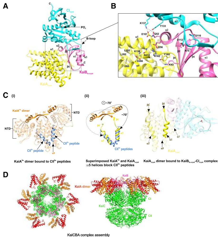
Fig. 7. KaiCBA ternary complex depicting the KaiA autoinhibition mechanism. a A 2.6-Å ternary complex between KaiA cryst and KaiB fs-cryst -Cl cryst (PDB 5JWR; KaiA cryst in yellow, KaiB fs-cryst in pink, and Cl cryst in cyan). b Enlarged view of the enclosed box in a depicting the binding interface of the ternary complex. Dashed lines show the electrostatic interactions. c Conformational changes in the KaiA dimer when sequestered into a KaiCBA complex. (i) Structure of KaiA in orange bound to CII peptides in blue (from S. elongates ; PDB 5C5E) highlighting the \alpha 5 and \alpha 5' helices and \beta 6 and \beta 6' strands of the two KaiA monomers. (ii) KaiA se (orange) and KaiA cryst in ternary complex (yellow) superimposed showing only the \alpha 5 and \alpha 5' helices and \beta 6 and \beta 6' strands. (iii) The Cl cryst -KaiB fs-cryst -KaiA cryst ternary complex. Panels (i), (ii), and (iii) highlight only the \alpha 5 and \alpha 5' helices and \beta 6 and \beta 6' strands of the two KaiA monomers depicting the structural basis of the mechanism of KaiA autoinhibition. d Top and side views of higher KaiCBA complex assembly (PDB 5N8Y) depicting the KaiC hexamer in green, the hexameric ring of KaiB monomers in pink, and KaiA homodimers in red and orange
