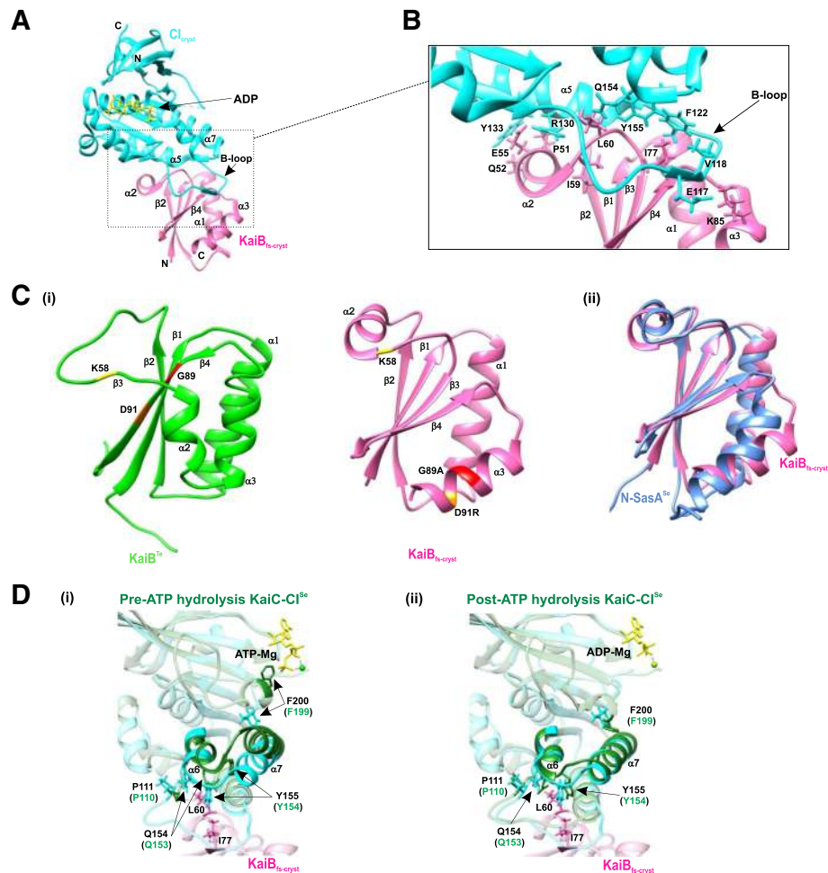
Fig. 5. Rare active fold-switched form of KaiB (fsKaiB) binds to the post-hydrolysis state of KaiC CI domain. a A 1.8-Å resolution structure of the KaiB fs-cryst -CI cryst complex (PDB 5JWO; from T. elongates ). The ribbon diagram shows KaiB fs-cryst in pink, CI cryst in cyan, and bound ADP in yellow. Enclosed dotted box depicts the binding interface between KaiB fs-cryst and CI cryst . b Enlarged view of the KaiB fs-cryst -CI cryst complex binding interface depicting the interacting residues. c Structural comparison of KaiB ground state (gs) and fsKaiB: (i) KaiB T E (gsKaiB; PDB 2QKE, subunit A) in green, KaiB fs-cryst in pink; (ii) superposition of KaiB fs-cryst in pink with N-SasA Se (PDB 1T4Y; Se: S. elongatus ) in cornflower blue. Residues K58, G89, and D91 are highlighted in yellow, red, and orange, respectively. d Comparison of the ATP binding site of the KaiB fs-cryst -CI cryst complex with ATP binding site of KaiC CI structures (from S. elongates ) in the pre- and post-hydrolysis states: superposition of ADP-bound CI cryst (cyan) with the CI Se structure (green) in the (i) pre-ATP hydrolysis state (PDB 4TLC, subunit C) and (ii) post-ATP hydrolysis state (PDB 4TLA, subunit E)
