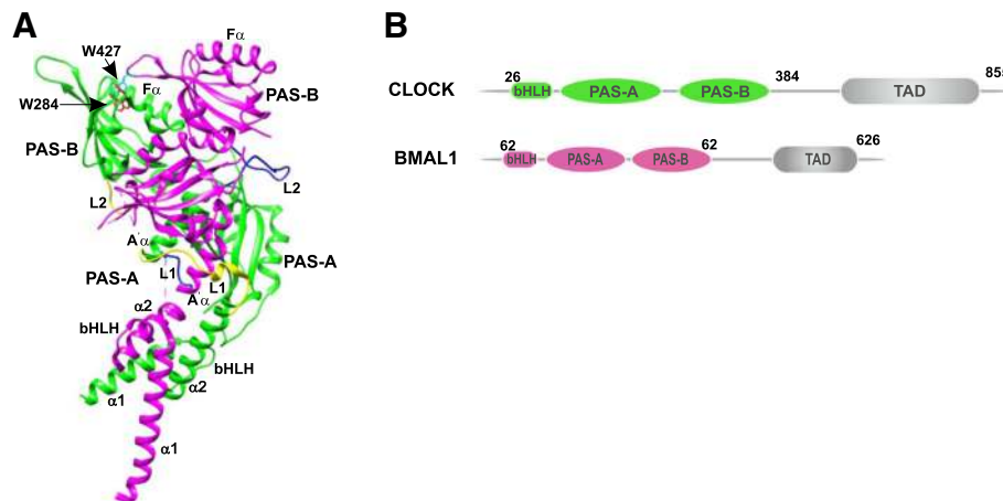
Fig. 10. Crystal structure of the mouse CLOCK–BMAL1 complex (PDB 4F3L). a The ribbon diagram of the complex shows the CLOCK subunit in green and BMAL1 in pink. Yellow and blue highlight the respective linker regions between the domains. b Domain architecture of CLOCK and BMAL1 depicting the basic helix-loop-helix domain and the two PAS domains
