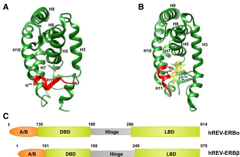
Fig. 11. Structure of Rev-erb \beta LBD monomer. a The apo form (green), without heme (PDB 2V0V), and b as a heme-containing (yellow) complex (PDB 3CQV), with the prosthetic group bound in the ligand-binding pocket. The conserved Cys384 (cyan) and His568 (red) residues involved in heme-binding are shown in stick representation. Helices H11 (red) and H3 undergo conformational changes to accommodate the heme prosthetic group. c The domain architecture of the Rev-erbs depicting the variable N-terminal A/B region (orange), DNA-binding domain (DBD) and the ligand-binding domain (LBD)
