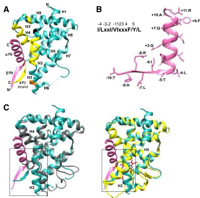
Fig. 12. Structure of N-CoR ID1 peptide and interactions. a N-CoR ID1CoRNR peptide (pink) bound to Rev-erb \alpha\Delta 323-423 LBD (sea green; PDB 3N00) depicting the N-CoR ID1 peptide \beta -strand ( \beta 1N) and \alpha -helix ( \alpha 1N) and the new C-terminal \beta -strand sY of Rev-erb \alpha LBD. The backbone of the contact residues in H3, H4, H5, and the new \beta -strand are shown in yellow and the supporting H3 residues in orange. b Representation of the amino acid residue positions in the N-CoR ID1 peptide defining the new extended motif for NRCOR. c Comparison of the N-CoR ID1 CoRNR peptide (pink) bound to Rev-erb \alpha\Delta 323-423 LBD (sea green) with apo-Rev-erb \beta (gray) and heme (red)-bound Rev-erb \beta (yellow). The region within the black box represents the changes in H3 as a result of conformational changes in H11 when Rev-erb binds to N-CoR ID1/heme.
