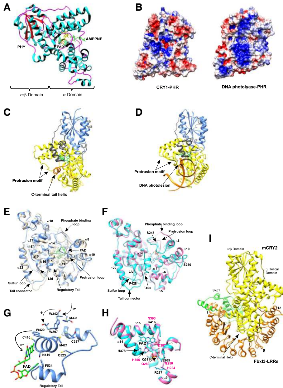
Fig. 16. a CRY1-PHR structure (PDB 1U3D) with helices in cyan, \beta -strands in red, FAD cofactor in yellow, and AMPPNP (ATP analogue) in green. b electrostatic potential in CRY1-PHR and E. coli DNA photolyase (PDB 1DNP). Surface areas colored red and blue represent negative and positive electrostatic potential, respectively. c dCRY (PDB 4JZY) and d 6-4 dPL (PDB 3CVU). The C-terminal tail of dCRY (orange) replaces the DNA substrate in the DNA-binding cleft of dPL. The N-terminal \alpha/\beta domain (blue) is connected to the C-terminal helical domain (yellow) through a linker (gray). FAD cofactor is in green. e Structural comparison of dCRY (blue; PDB 4JZY) with dCRY (beige; PDB 3TVS, initial structure; 4GU5, updated) [308, 309]. Significant changes are in the regulatory tail and adjacent loops. f Structural comparison of mCRY1 (pink; PDB 4K0R) with the dCRY (cyan; PDB 4JZY) regulatory tail and adjacent loops depicting the changes. Conserved Phe (Phe428 dCRY and Phe405 mCRY1 ) depicted that facilitates C-terminal lid movement. g dCRY photoactivation mechanism: Trp342, Trp397, and Trp290 form the classic Trp e^- transfer cascade. Structural analysis suggest the involvement of the e^- rich sulfur loop (Met331 and Cys337), the tail connector loop (Cys523), and Cys416, which are in close proximity to the Trp cascade in the gating of e^- s via the cascade. h Comparison of the FAD binding pocket of dCRY (cyan) and mCRY1 (pink). Asp387 mCRY1 occupies the binding pocket. The mCRY1 residues (His355 and Gln289), corresponding to His 378 and Gln311 in dCRY, at the pocket entrance are rotated to "clash" with the FAD moiety. Gly250 mCRY1 and His224 mCRY1 superimpose Ser265 dCRY and Arg237 dCRY , respectively. i Crystal structure of the complex (PDB 4I6J) between mCRY2 (yellow), Fbx13 (orange), and Skp1 (green). The numbers 1, 8, and 12 display the position of the respective leucine rich repeats (LRR) present in Fbx13
