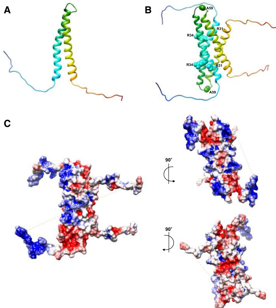
Fig. 13. Predicted structural models of ELF4. The a ELF4 monomer, b ELF4 dimer, and c electrostatic potential surface calculated for the ELF4 dimer. Surface areas colored red and blue represent negative and positive electrostatic potential, respectively
