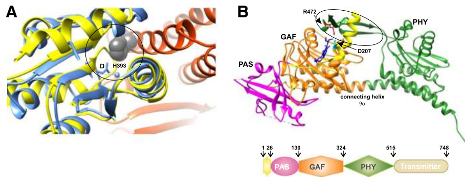
Fig. 14. Structure of the PsR domain of CikA. a CikA-PsR (yellow, PDB 2J48) superimposed on the Spo0F–Spo0B complex (blue and orange, PDB 1F51) depicting the structural difference in the HPK–PsR domain interaction interface in CikA and bacterial Spo0F–Spo0B. b The complete phytochrome sensory module of Synechocystis 6803 Cph1 (PDB 2VEA). The tongue region is encircled. The N-terminal region is shown in yellow, the PAS domain in pink, the GAF domain in orange, and the PHY domain in green. The phycocyanobilin (PCB) chromophore is shown in blue stick representation
