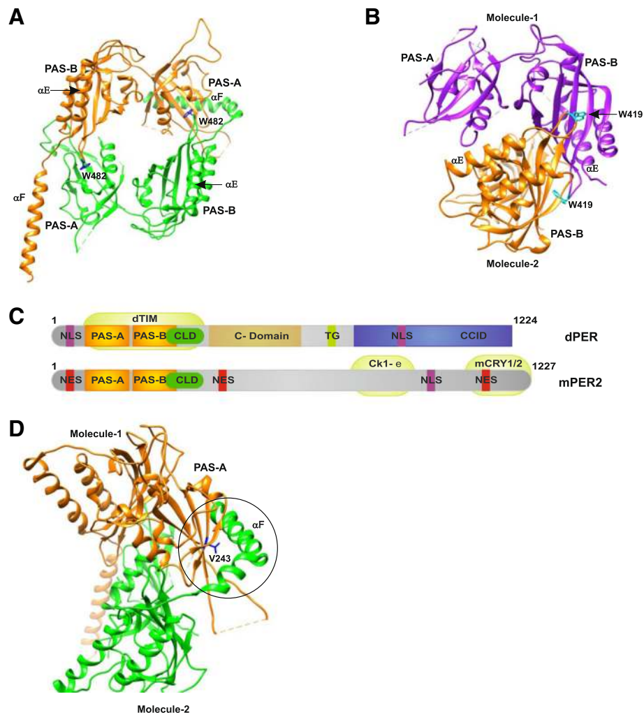
Fig. 8. Crystal structures of the period proteins. a dPER (PDB 1WA9) and b mPER2 (PDB 3GDI) dimers in cartoon representation. The conserved Trp482 (dPER, dark blue) and Trp419 (mPER2, cyan) residues are shown in stick representation. c The domain architecture of dPER and mPER2 proteins. The two PAS domains (PAS-A and PAS-B), the cytoplasmic localization domain (CLD, green), the conserved C-domain (light brown), nuclear localization signals (NLS, purple), NES (red), the threonine-glycine (TG) repeat region, and the dCLK:CYC inhibition domain (CCID, blue) of dPER and/or mPER2 are shown. CK1e, mCRY1/2, and dTIM are shown at their binding sites. d dPER structure representing the PAS-A- \alpha F interaction (encircled region) interface and depicting the location of V243 (blue)
