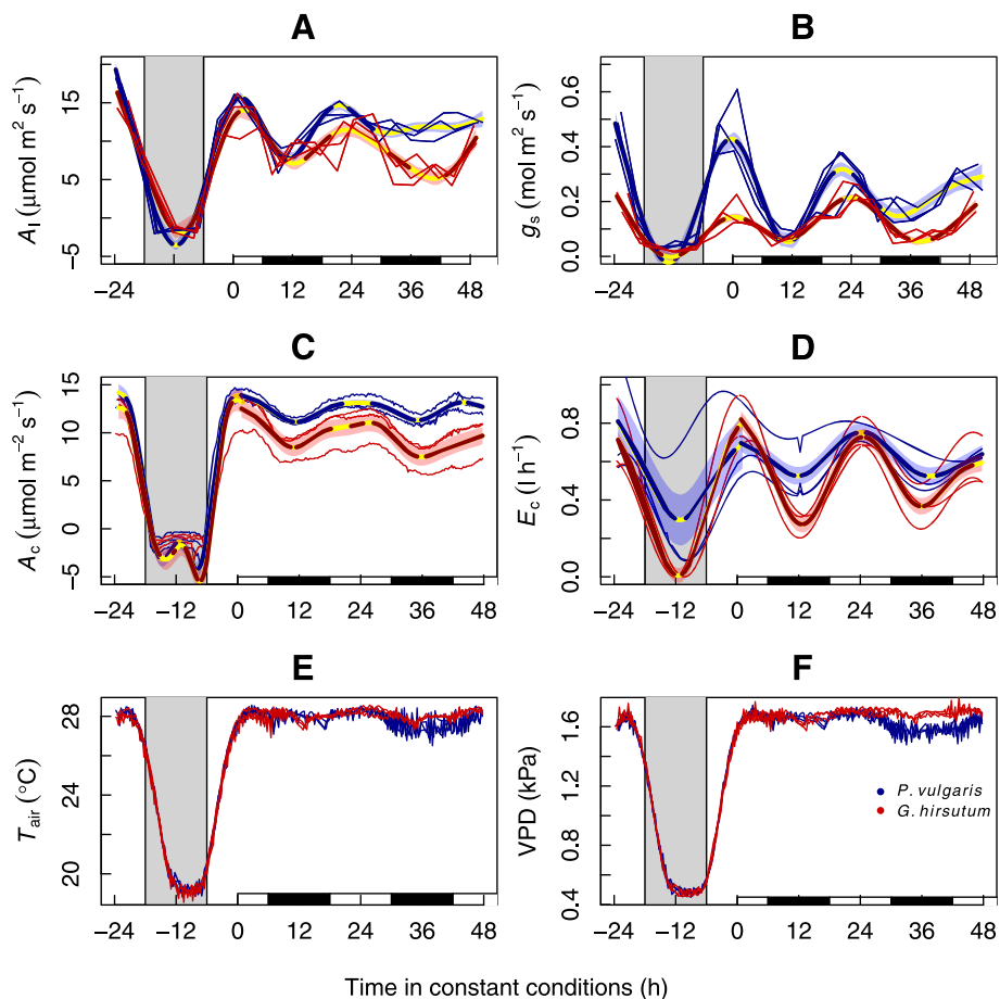
Fig. 1 Circadian regulation of leaf and canopy-scale CO 2 and H 2 O fluxes. We grew cotton ( Gossypium hirsutum ) and bean ( Phaseolus vulgaris ) in experimental macrocosms at the Montpellier European Ecotron. During experimental conditions, temperature ( T_{\text{air}} , e ) and vapor pressure deficit (VPD, f ) mimicked the environmental conditions of an average August day in Montpellier, with 500 \mu\text{mol m}^{-2} \text{s}^{-1} photosynthetically active respiration (PAR) (first 24 h shown) remaining constant for the following 48 h starting at solar noon. Grey or white background indicate when PAR was at or above 0 \mu\text{mol m}^{-2} \text{s}^{-1} respectively. The white and black rectangles at the base indicate the subjective day (when it would have been daytime during entrainment) and subjective night, respectively, under constant conditions. Thin lines represent measured values at each of three replicate macrocosms, and thick lines (and shaded error intervals) indicate the prediction (and SE) of generalized additive mixed model (GAMM) fitting separately for each species (some lines may overlap). Portions of the thick line in yellow indicate lack of statistical variation in the slope. Significant variation (GAMM best-fit line portions not yellow) in leaf ( a ) and canopy ( c ) carbon assimilation ( A_l and A_c , respectively), stomatal conductance ( g_s , b ) and canopy transpiration ( E_c , d ) prevailed for all fluxes and processes, at least in the first 24 h under constant conditions. This can be fully attributed to circadian action. Clock regulation is plastic and may relax after prolonged exposures to constant conditions [56]. Negative dark-time values of A_l/g_s and A_c/E_c were cropped as they lack biological meaning
