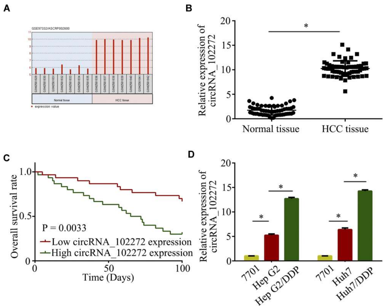
Figure 1 CircRNA_102272 is upregulated in HCC tissues and cells. (A) GEO dataset (GSE97332) showed that circRNA_102272 is significantly increased in HCC tissues compared to normal tissues. (B) CircRNA_102272 expression was significantly increased in HCC tissues compared to normal tissues. (C) Survival rates were examined by Kaplan–Meier analysis in HCC patients. (D) CircRNA_102272 expression was significantly increased in HCC cells compared to normal cells. The data shown represent the mean \pm SD. * p < 0.05 .
