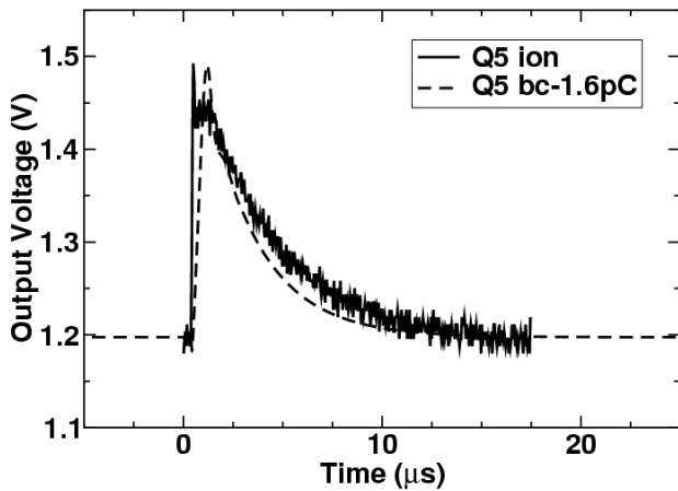
Fig. 8 (b) Comparison of SETs observed at the output of the LM124. The experimental curve “ion” was obtained by exposing transistor Q5 to the ion microbeam. The simulated curve indicates the junction and the charge that needs to be injected to match the experiment.
