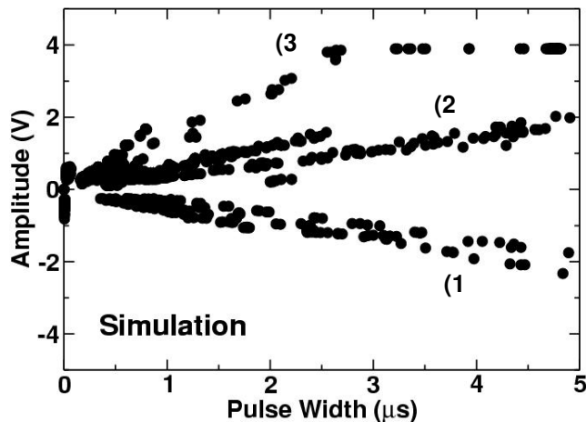
Fig. 11 Simulations results of laser-calibrated model plotting amplitude vs. time-width at half maximum of amplitude (FWHM) of observed output voltage transients. The integrated charge of the current sources used to produce the stimuli was varied from 0.1 to 10pC.
