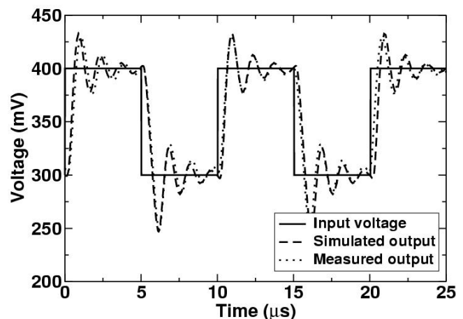
Fig. 4 Comparison between measured and simulated LM124 small signal pulse response.
