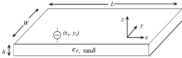
Fig. 3. Typical rectangular power bus structure.
