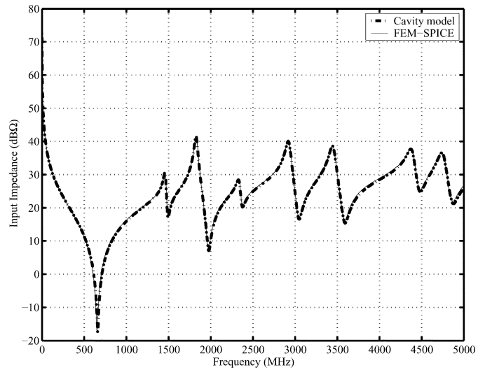
Fig. 4. Calculated input impedance using cavity model and FEM-SPICE for Problem 1.
