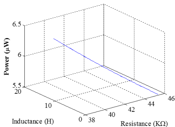
Figure 11. Variation of output power based on load resistance and inductance in IL circuit
