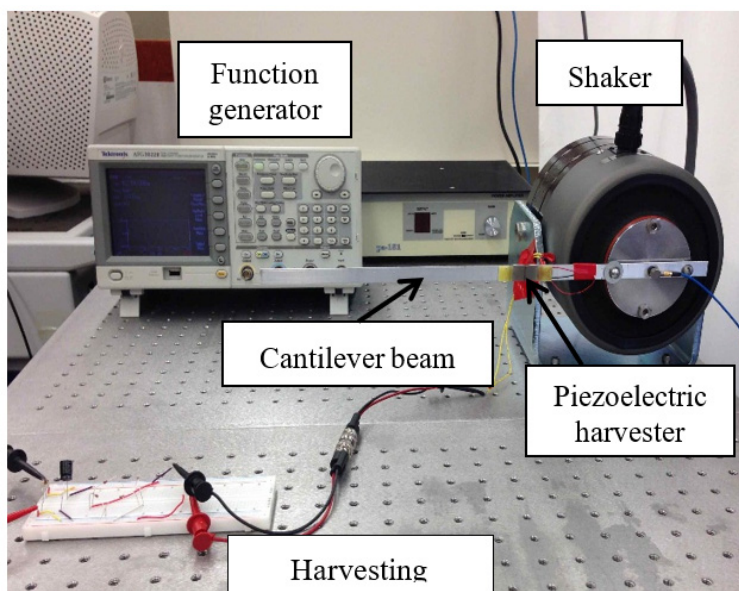
Figure 14. Experimental setup for the piezoelectric harvester attached on the cantilever beam (Zargarani & Mahmoodi, 2017)
