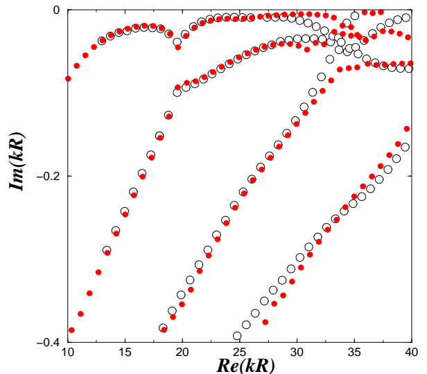
FIG. 6: Comparison between perturbation and numerical spectra for the cut disk with \epsilon = 0.05 . Open black circles are results of the direct numerical simulations and red full circles correspond to the perturbation expansion (33).
