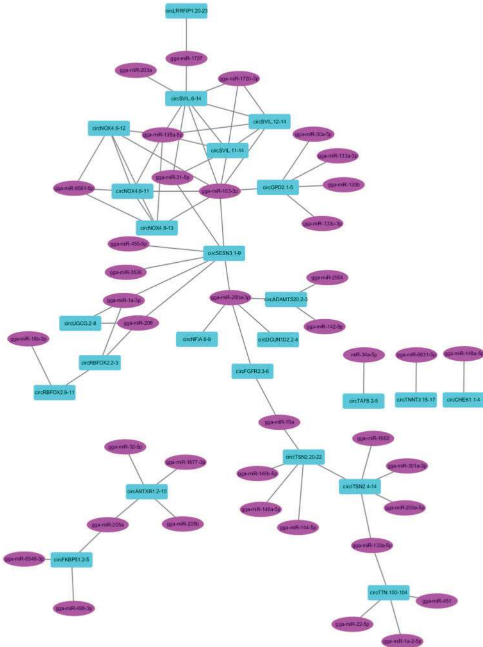
Figure 3. Interaction network of circRNA and their potential target miRNAs. The top 20 differentially expressed exonic circRNAs of each comparison group and their potential target miRNAs were used for their interaction network analysis. Rectangle nodes represent circRNAs and circle nodes represent miRNAs.
