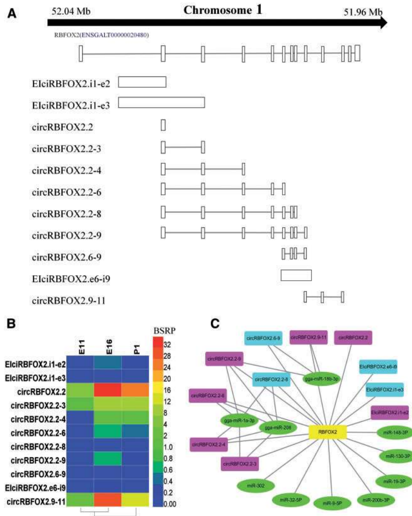
Figure 4. Annotation of circular RBFox2 gene. (A) All circRNA isoforms of the RBFox2 gene in chicken embryonic muscle. (B) The abundance of circular RBFox2 in chicken embryonic muscle. The scale bar 0–32 represents the abundance of circRNAs (BSRP value). (C) Network of circular RBFox2 with miRNAs. Dark gray rectangle nodes represent highly-expressed circRNAs, light gray rectangle nodes represent low expressed circRNAs and circle nodes represent miRNAs.
