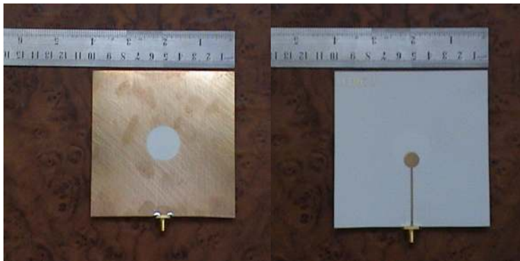
Figure 1. (a) Antenna geometry, (b) Photograph — left handed: circular slot, right handed: feed network.
