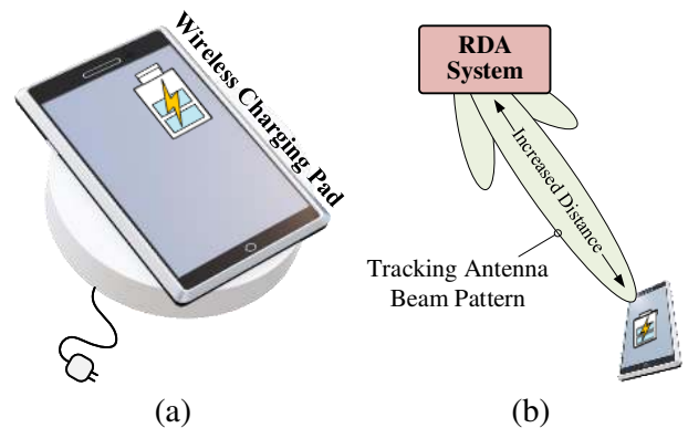
Fig. 1. Conventional WPT by inductive coupling (a), and the proposed WPT approach using retrodirective antenna (RDA) technology (b) where the device can be tracked and its battery charged in free-space at an increased distance.
