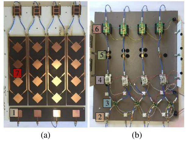
Fig. 4. Picture of the developed RDA system. Front (a), back (b) and schematic of one of the four RF chains (c). The components used in the antenna system for each RF chain: (1) 2.5 GHz RHCP corner clipped patch (part of the 4 \times 1 receiver array), (2) band pass filter from TriQuint 885009 at 2.5 GHz, (3) mixer from Linear Technology LTC5549, (4) driver amplifier from MiniCircuits ZFL-2500+, (5) band pass filter from TriQuint 885017 at 2.4 GHz, (6) power amplifier from TriQuint TQP9111 and (7) 2.4 GHz LHCP 4 \times 1 sub-array (part of the 16 element transmitter array).
