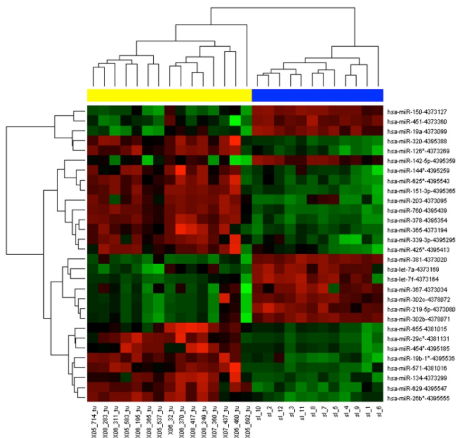
Figure 1 Hierarchical clustergram iscriminating blood serum of RCC patients and healthy controls according to diferentially expressed miRNAs (yellow color indicate serum samples of RCC patients, blue healthy controls, p < 0.0001 ).
