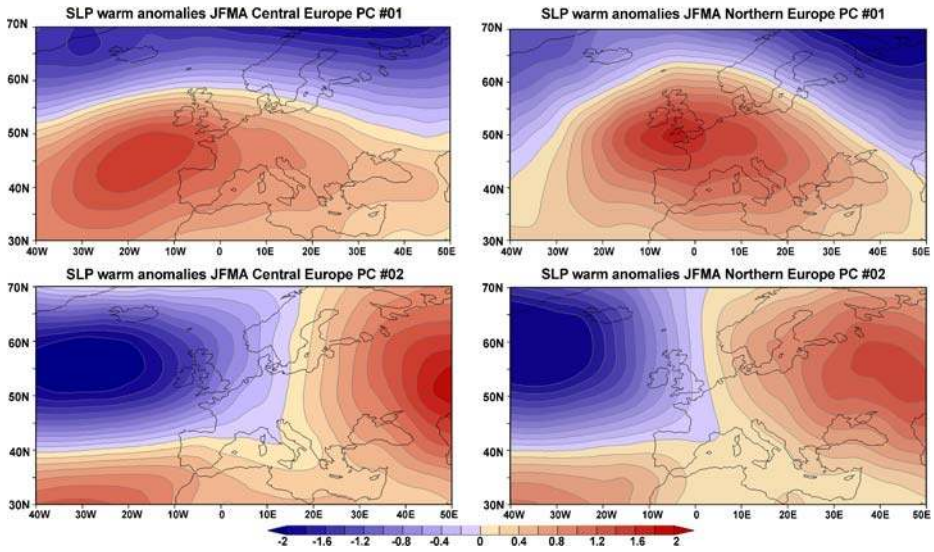
Fig. 2 Major circulation patterns associated with warm JFMA seasons in Central Europe ( left ) and Northern Europe ( right ) over the 1760–2007 period, derived from objectively reconstructed SLP fields (developed in Jacobeit et al. 1998; normalized T-mode PCA scores). The regions in blue ( red ) colours show low ( high ) pressure systems. The explained variance for the two PCs for Central Europe is 61.3% and 34.1%; for Northern Europe it is 39.2% and 35.6%
