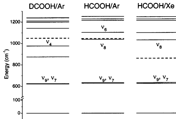
FIG. 4. Vibrational level structure of trans HCOOH and trans DCOOH as determined from their infrared spectra. The energy of the ground state of cis FA estimated by using the gas-phase energetics (Ref. 7) and ab initio calculated solvation energies for the two conformers is shown with a dashed line. The labels for selected vibrational states correspond to torsion ( \nu_9 ), OCO scissor ( \nu_7 ), C–H out-of-plane wag ( \nu_8 ), C–D rocking ( \nu_4 ), and COH–CO deformation ( \nu_6 ) modes (Ref. 9).
