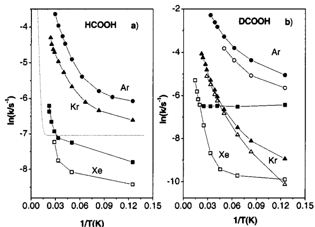
FIG. 3. Arrhenius plots for tunneling of (a) HCOOH and (b) DCOOH in various matrices. Data for two representative sites for each host are shown as solid and open symbols. The data for two sites shown in plot (a) for Xe as solid and open squares correspond to labels A and B in Fig. 2, respectively. For comparison, a simulated temperature dependence for tunneling from two lowest intramolecular vibrational states is shown as a dotted line.
