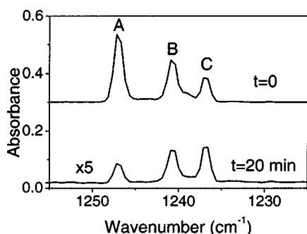
FIG. 2. IR absorption of cis -HCOOH in the CO-COH deformation fundamental region in solid Xe at 8 K. A, B, and C denote the absorptions corresponding to various sites (local environment). The lower trace was measured 20 min after the upper trace showing the different tunneling rates for the three sites.
