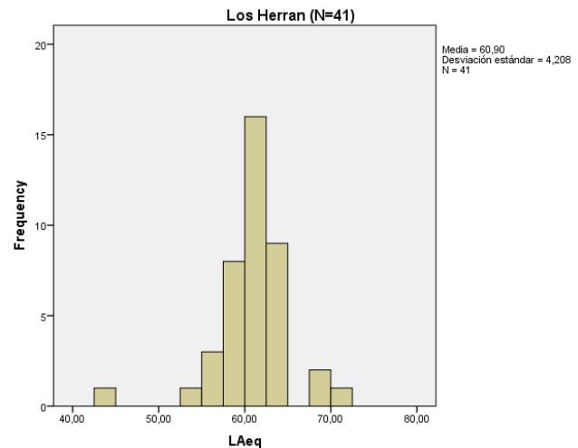
Figure 5: Noise levels measured in all the observation made in one place. A total of 41 observations were developed.
