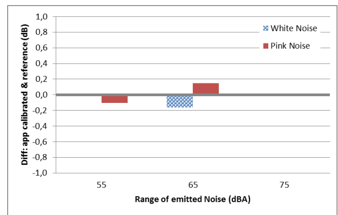
Figure 4: Difference: app calibrated and reference.
