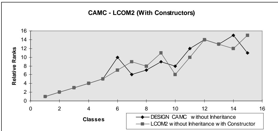
Figure 2. Plot of the CAMC and LCOM2 Rankings of the 15 Classes in Table 3
