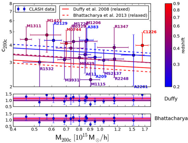
Figure 11. This figure is identical to Figure 10 but shows the c - M relations derived from the relaxed samples of D08 and B13 .
