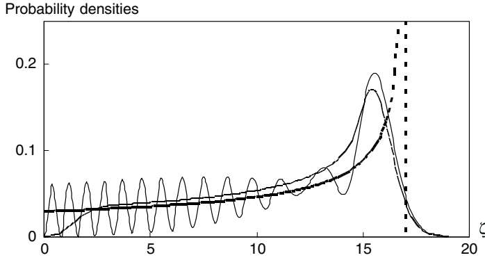
Figure 5. Classical ( P_{cl}(\zeta) , dotted curve) and quantum ( P_{qu}^{(0)}(\zeta) , dashed curve, and P_{qu}^{(3)}(\zeta) , C_{14} = 0.5065 , C_{15} = 0.6129 , C_{16} = 0.4611 , solid curve) position probability densities.
