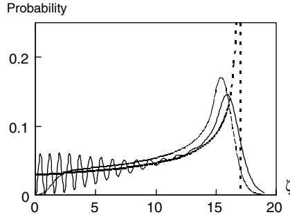
Figure 6. Classical ( P_{cl}(\zeta) , dotted curve) and quantum ( P_{qu}^{(0)}(\zeta) , dashed curve, and P_{qu}^{(7)}(\zeta) , C_{12} = 0.1316 , C_{13} = 0.2980 , C_{14} = 0.5065 , C_{15} = 0.6129 , C_{16} = 0.4611 , C_{17} = 0.1118 , C_{18} = -0.1224 , solid curve) position probability densities.
