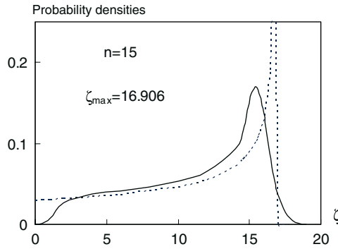
Figure 2. Classical, P_{cl}(\zeta) , dotted curve, and zero approximation quantum, P_{qu}^{(0)}(\zeta) , solid curve, position probability densities. \zeta = x \left( \frac{2m^2g}{\hbar^2} \right)^{1/3} .
