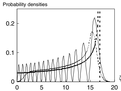
Figure 4. Classical ( P_{cl}(\zeta) , dotted curve) and quantum ( P_{qu}^{(0)}(\zeta) and P_{qu}^{(st)}(\zeta) , for a particle in quantum stationary state n = 15 , solid curves) position probability densities.
