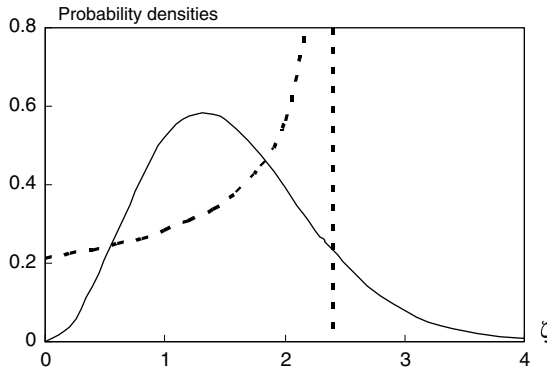
Figure 3. Classical ( P_{cl}(\zeta) , dotted curve) and quantum ( P_{qu}^{(st)}(\zeta) , for a particle in quantum stationary state n = 0 , solid curve) position probability densities.
