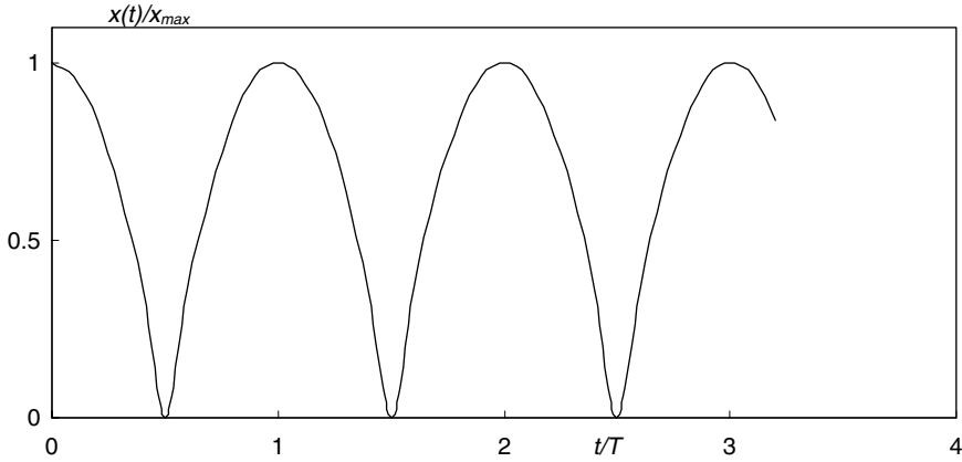
Figure 1. Trajectory of particle motions in the gravitational field.
