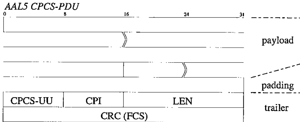
Fig. A.3. AAL5 CPCS-PDU
