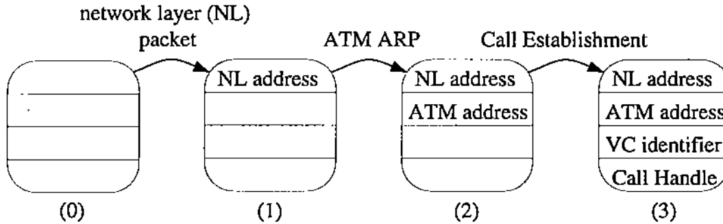
Fig. 5. Example for a complete resolution process. This graph is only a small subset of the real automaton
