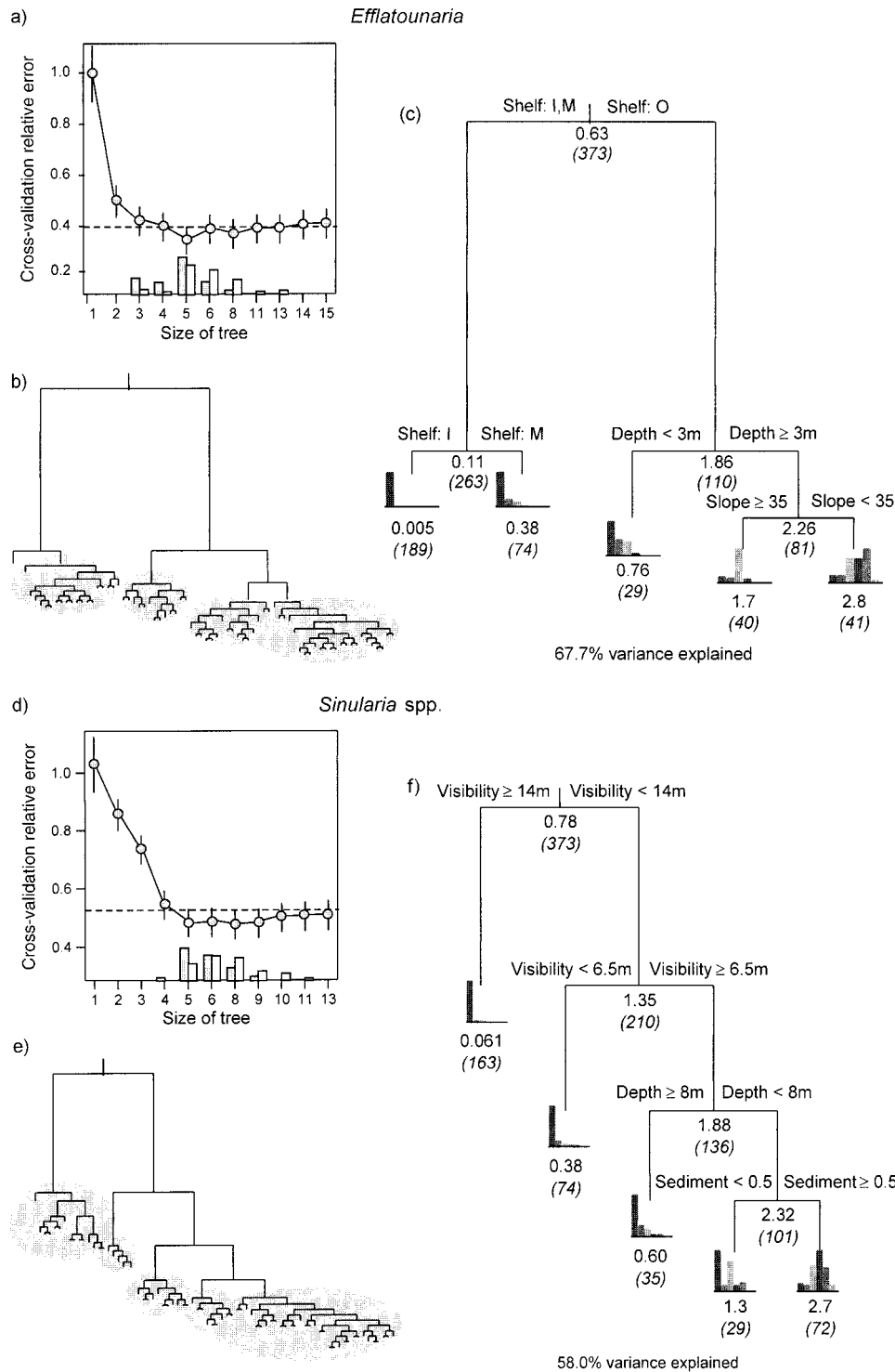
FIG. 5. Regression trees explaining the abundances of the soft coral taxa Eflatounaria , Sinularia spp., and Sinularia flexibilis in terms of the four spatial variables (shelf position, location, reef type, and depth) and four physical variables (sediment, visibility, waves, and slope). At the bottom of the cross-validation plots (a, d, g), the bar charts show the relative proportions of trees of each size selected under the 1-SE rule (gray) and minimum size rules (white) from a series of 50 cross-validations. For Eflatounaria (a), a five-leaf tree is most likely by either the 1-SE or the minimum rule. For Sinularia spp. (d), five to eight-leaf trees have support, and for S. flexibilis (g), five- to nine-leaf trees have support. Cross-validation plots (a, d, g), representative of the modal choice for each taxa according to the 1-SE rule, are also shown. For all three taxa, a five-leaf tree was selected (c, f, i). The shaded ellipses enclose nodes pruned from the full trees (b, e, h), each of which accounted for >99% of the total ss.
