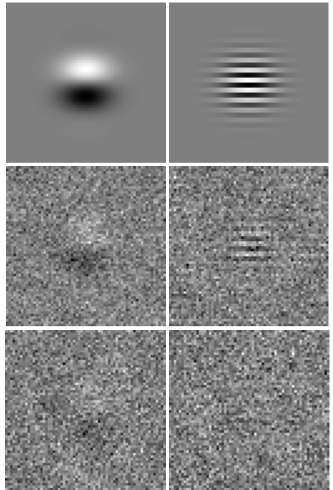
Figure 2. Top. Gabor signals with spatial frequencies of 2 cpd (left) and 16 cpd (right). Center. Classification images for the signal trials with the 2-cpd target (left) and the 16-cpd target trials (right). Bottom. Classification images for the no-signal trials with the 2-cpd target (left) and the 16-cpd target (right). The observer was C.S., who ran 5,900 trials at 2 cpd and 8,000 trials at 16 cpd (Ahumada & Beard, 1999).
