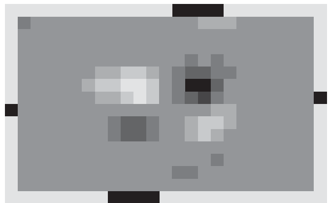
Figure 1. A raw classification image (top) and the same image smoothed and quantized (bottom), so only weights significantly different from zero are colored differently from the gray background. The black squares on the sides show the heights and positions of the fixed line (left) and the variable line offset (right). The dark lines on the top and bottom show the lengths and positions of the lines. The observer was A.J.A., who ran 1,600 trials (Ahumada, 1996).
