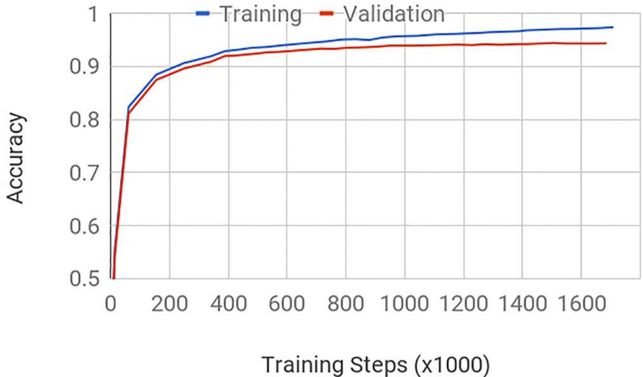
Fig 2. Classifier accuracy. Accuracy on the training and validation sets as a function of the number of steps of training. Training halts when the performance on the evaluation set no longer increases ('early stopping'). As is typical for this type of stochastic training, performance increases rapidly at first as large training steps are taken, and slows down as the learning rate is annealed and the model fine-tunes its weights.
