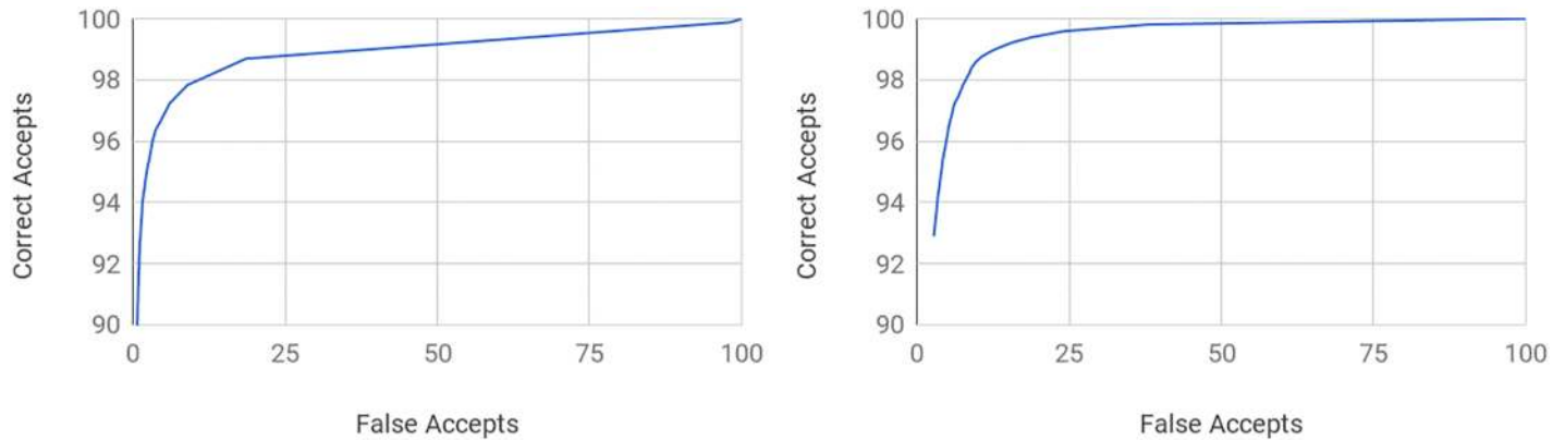
Fig 3. Receiver operating characteristic curves. (A) Percentage of the correctly accepted detection of crystals as a function of the percentage of incorrect detections (AUC: 98.8). 98.7% of the crystal images can be recalled at the cost of less than 1% false positives. Alternatively, 94% of the crystals can be retrieved with less than 1.6% false positives. (B) Percentage of the correctly accepted detection of precipitate as a function of the percentage of incorrect detections (AUC: 98.9). 99.6% of the precipitate images can be recalled at the cost of less than 25% false positives. Alternatively, 94% of the precipitates can be retrieved with less than 3.4% false positives.
