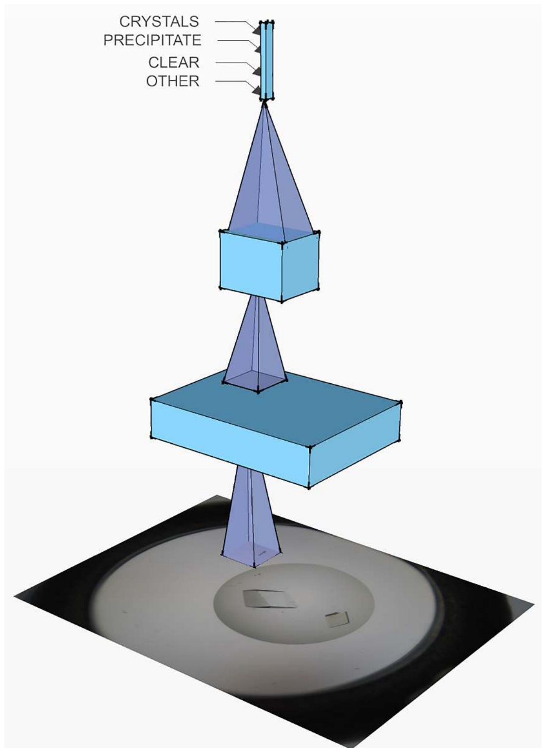
Fig 1. Conceptual representation of a convolutional neural network. A CNN is a stack of nonlinear filters (three filter levels are depicted here) that progressively reduce the spatial extent of the image, while increasing the number of filter outputs that describe the image at every location. On top of this stack sits a multinomial logistic regression classifier, which maps the representation to one probability value per output class (Crystals vs. Precipitate vs. Clear vs. Others). The entire network is jointly optimized through backpropagation [33], in general by means of a variant of stochastic gradient descent [34].
