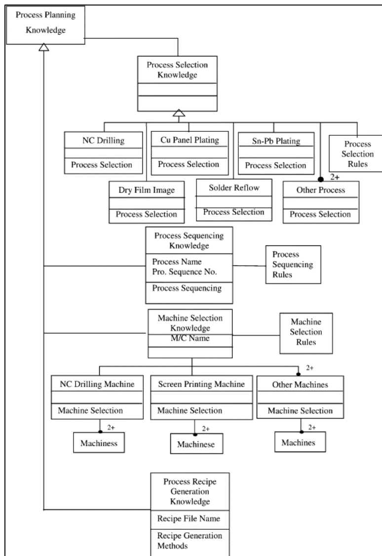
Figure 3: Object representation of the planning knowledge for manufacturing of printed circuit boards process planning Source: Law et al. (2001).
