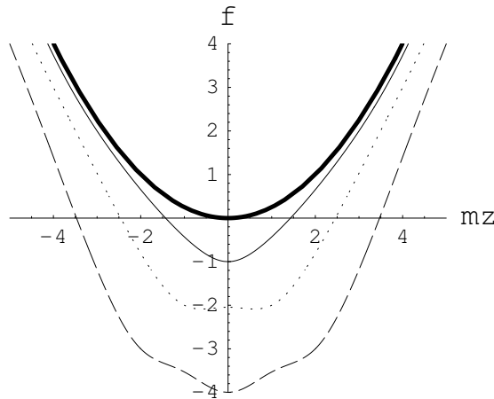
Figure 5: The thick line ( m_z^2 = 4f ) is the buckling curve for a rod of infinite length; while the plain, dotted, dashed curves are the curves of the 1st, 2nd and 3rd (resp.) buckling modes for a finite rod (eq. (22)).
