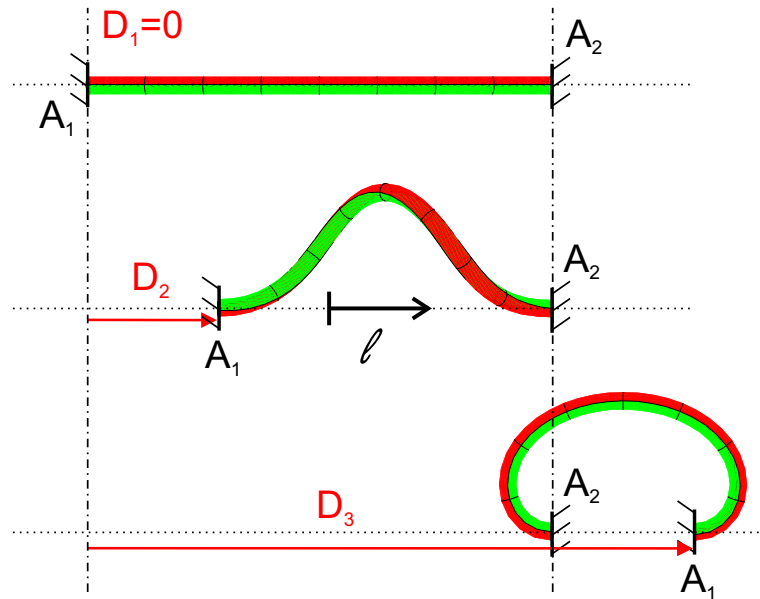
Figure 1: A rod with clamped boundary conditions: the axis \ell (joining point A_1 to point A_2 ) and the tangent of the rod at both ends are aligned. The end-shortening D_i of a configuration is the distance between the point A_1 in that configuration and the point A_1 in a straight configuration: D_1 = 0 , 0 < D_2 < L and L < D_3 < 2L .
