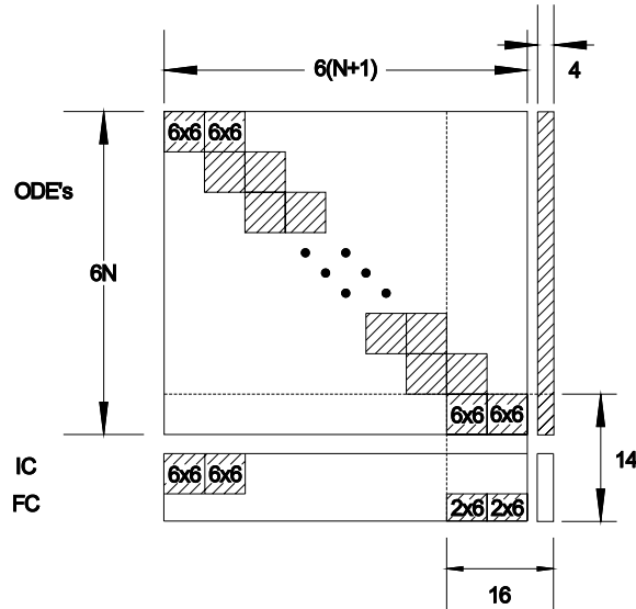
Figure 2: The block structure of the Jacobian F_u . IC stands for initial conditions. FC stands for final conditions
