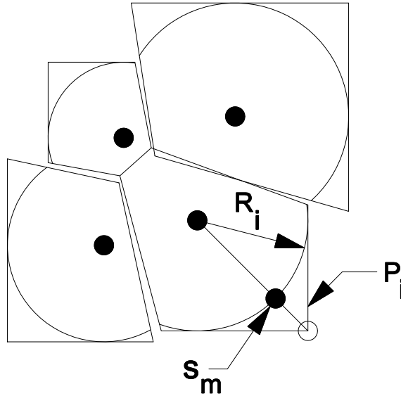
Figure 3: The basis of the continuation: a new tile is added for any u_i whose polygon P_i has a vertex outside |s| = R_i . The new tile is centered at a point which is the projection onto F = 0 of the intersection of a line between the origin and the exterior vertex and the circle |s| = R_i . The figure represents the projection of nearby tiles into the tangent space at u_i .
