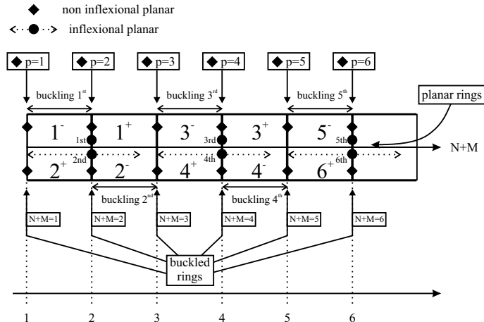
Figure 7: Sketch of the disposition of the different layers of the post-buckling surface together with important special paths of solutions (corresponding to planar or closed configurations). The harmonics are sorted according to their \Omega = N + M value. The borders that part the different harmonics are the buckled rings that appear for integer value of \Omega and the twisted planar rings that exist for continuous value of \Omega . All planar configurations but even inflexional ones have an integer \Omega . Above (resp. under) the line of planar twisted rings, u_- > u_0 (resp. u_- < u_0 ) and u_- = u_0 on the line.
