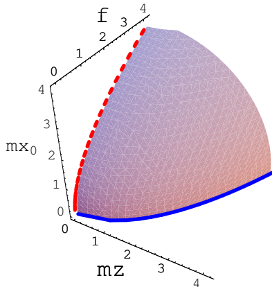
Figure 6: Post-buckling surface in the case of infinite length (homoclinic orbit). The surface is joining the buckling curve (plain blue, \theta_0 = 0 ) to the planar curve (dotted red, \theta_0 = \pi ).
