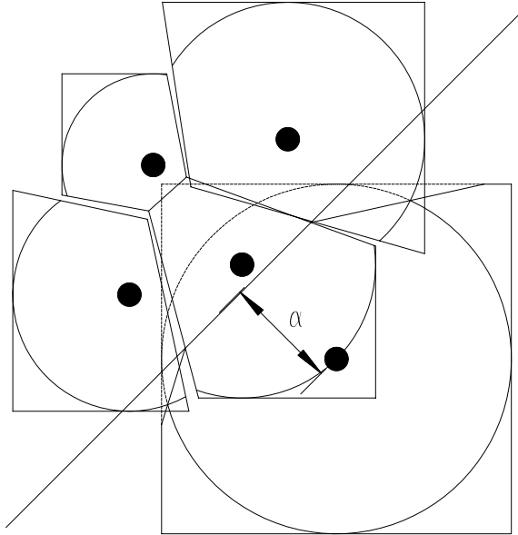
Figure 4: Updating the polygons: one halfplane is removed for each overlapping point. Again, the figure represents the projection of nearby points and polygons into the tangent space at u_i . If the manifold were flat the half spaces defined by \alpha_{im} and \alpha_{mi} are complementary, so there would be no gap between the polygons.
